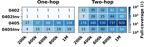
Figure 8: Minimum full-coverage retrieval depth ( k ) (for book B_1^c under NOLiMA). Lower ( \downarrow ) values are better.
