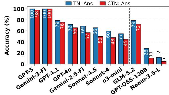
Figure 6: TN vs. CTN Ans accuracy under EBG prompting. We report an accuracy for the same runs whose Ans+Evid accuracy appears in Figure 3. Higher (↑) values indicate better performance.
