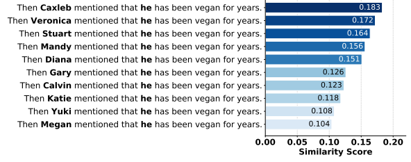
Figure 9: Ranking of the 0405 needle instantiated with 10 different character names based on cosine similarity to a one-hop test query. Although the sentence semantics remain unchanged, similarity scores vary across character tokens. Higher ( \uparrow ) values are better.
