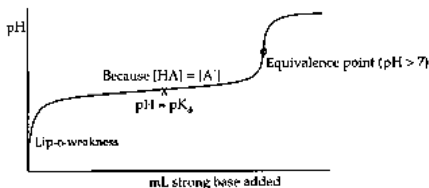
Case 2a: Weak acid titrated by a strong base
