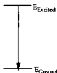
Electronic Transition (no vibrational transitions)
