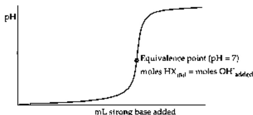
Case 1a: Strong acid titrated by a strong base
