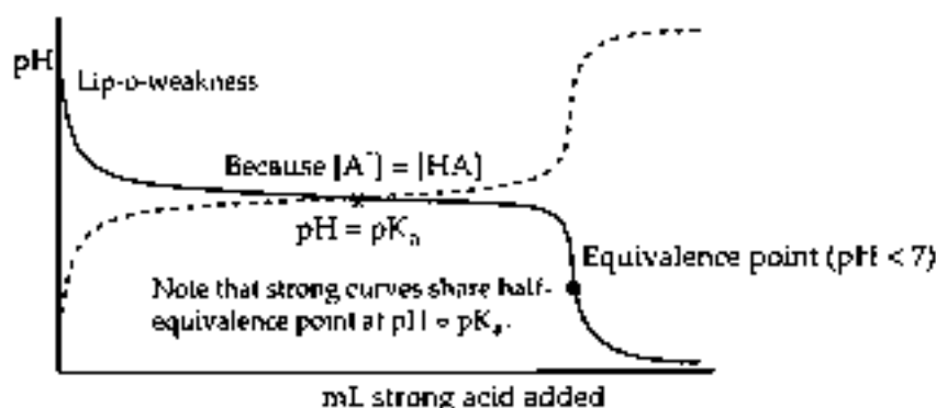
Case 2b: Weak base titrated by a strong acid
