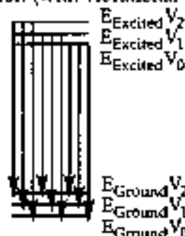
Electronic Transition (with vibrational transitions)
