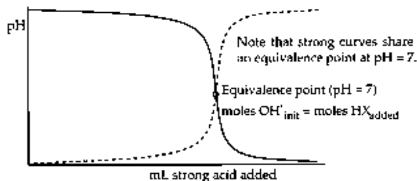
Case 1b: Strong base titrated by a strong acid
