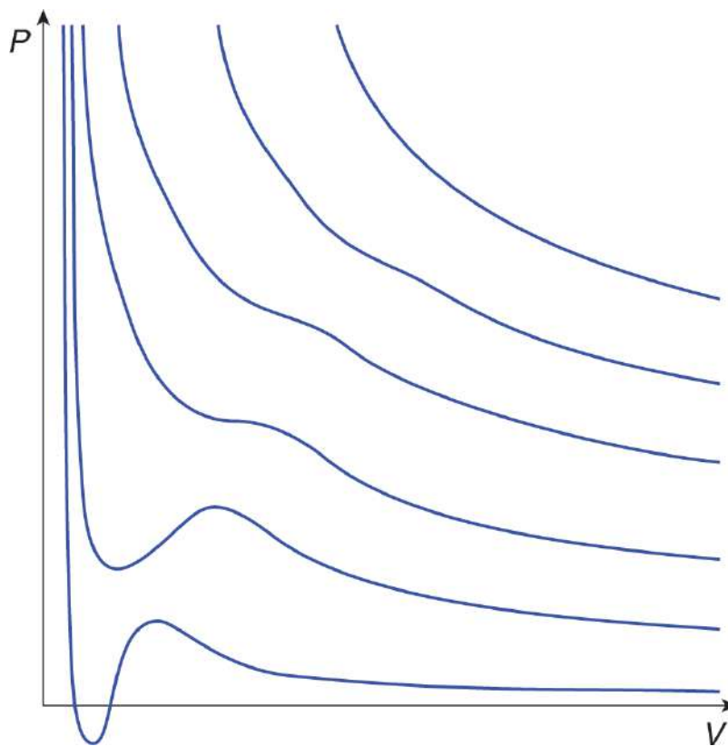
Figure 8.11. Real Gas Isothermal Curves
