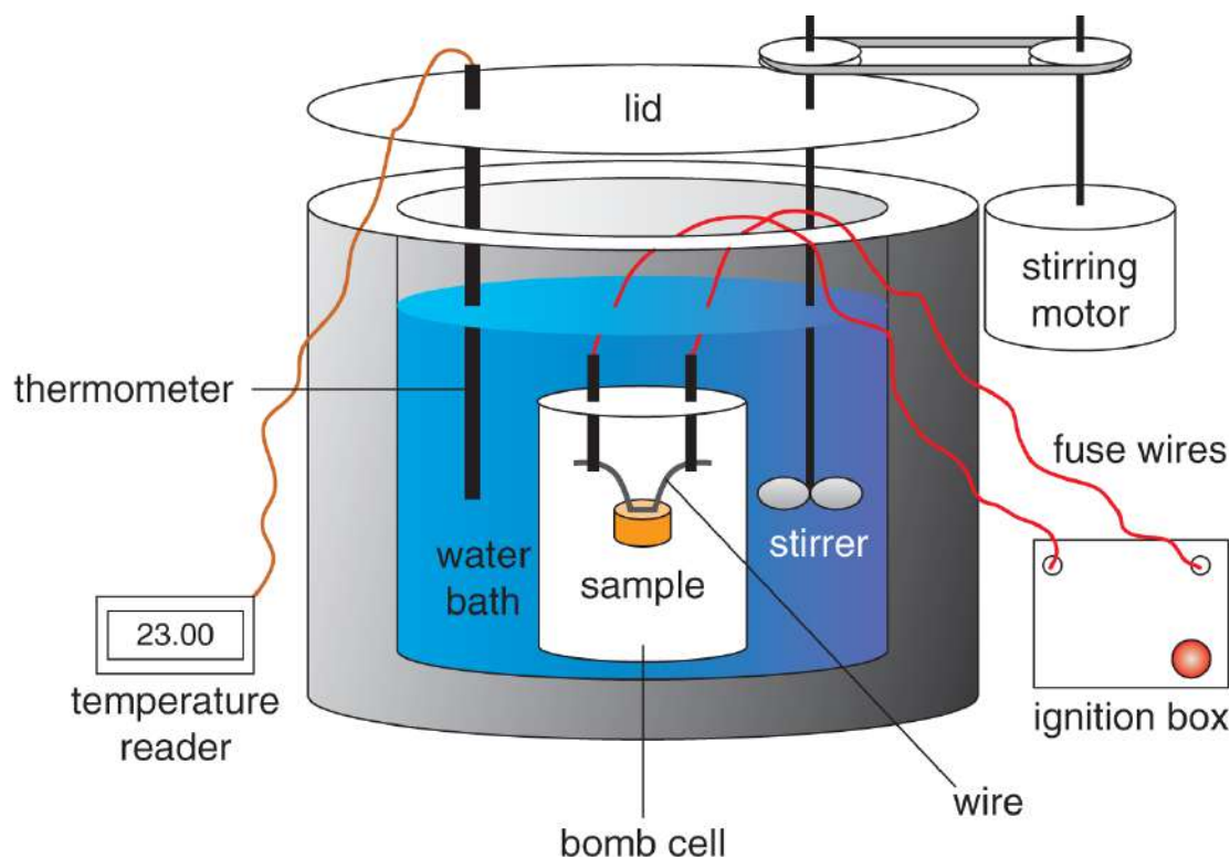
Figure 7.6. Diagram of a Bomb Calorimeter
