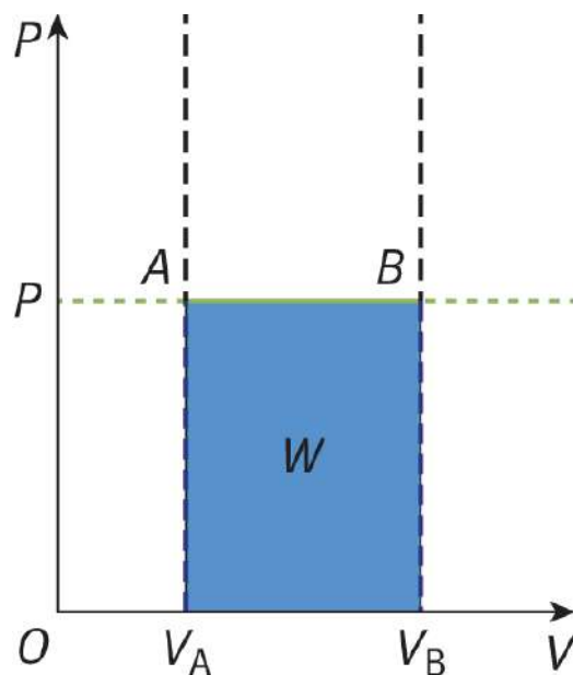
Figure 7.3. Graph of an Isobaric Expansion
