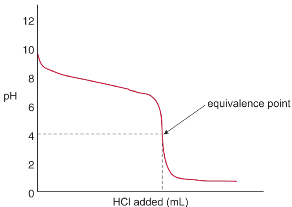
Figure 10.11. Strong Acid and Weak Base Titration Curve
