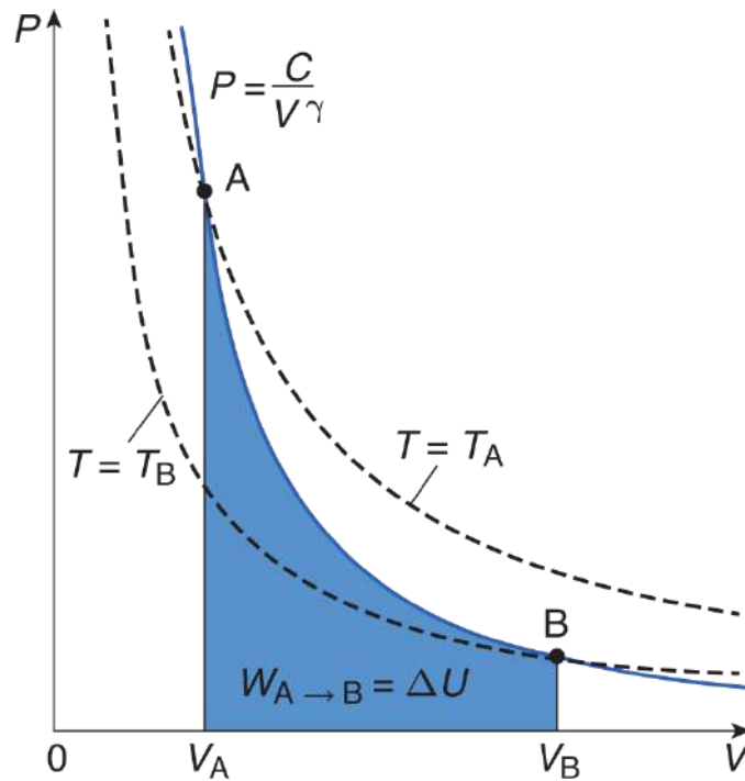
Figure 7.2. Graph of an Adiabatic Expansion
