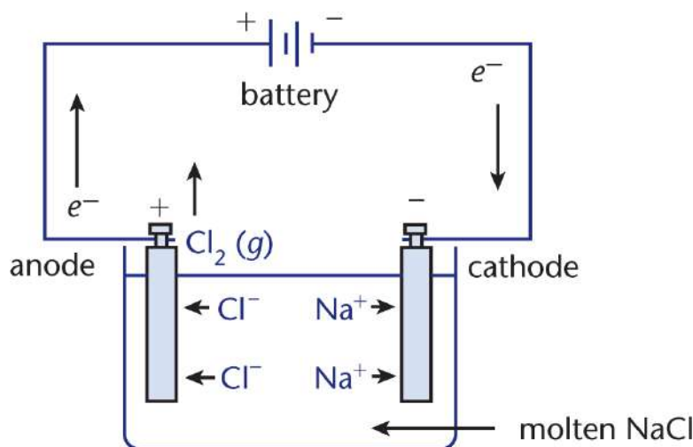
Figure 12.2. Electrolysis of Molten NaCl
