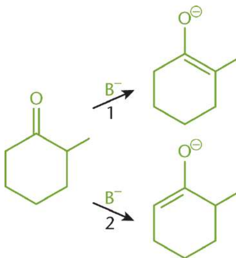
Figure 6.5. Conversion of 2-methylcyclohexanone to (1) Thermodynamic Product and (2) Kinetic Product
