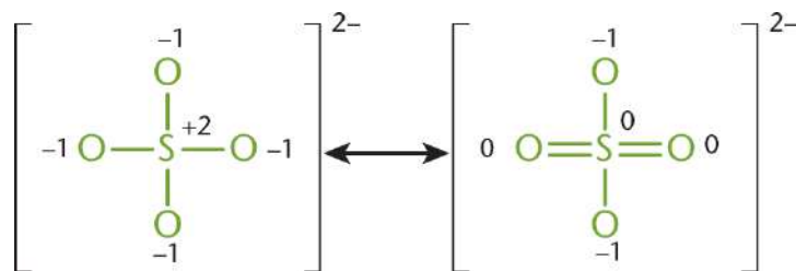
Figure 3.9. Two Different Resonance Forms of the Sulfate Ion
