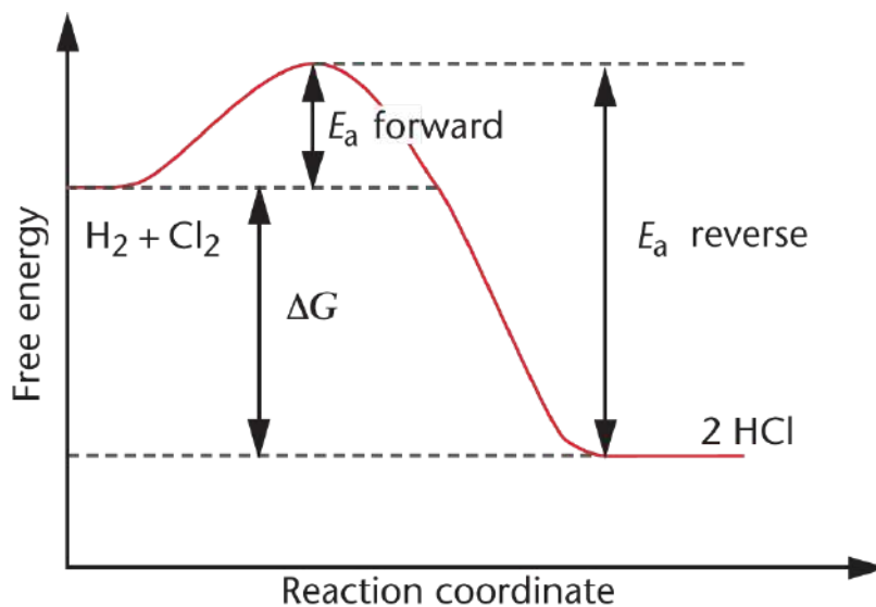
Figure 5.4. Reaction Diagram for the Formation of HCl
