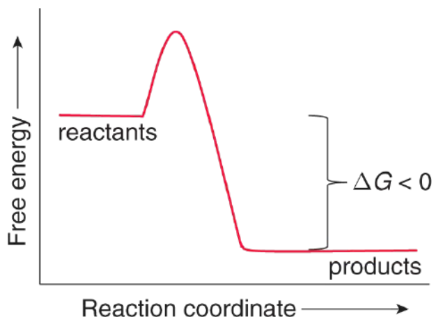
Figure 7.12. Exergonic Reaction Profile
