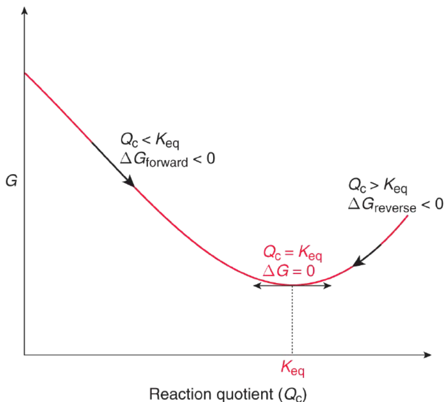
Figure 6.2. Gibbs Free Energy vs. Reaction Quotient
