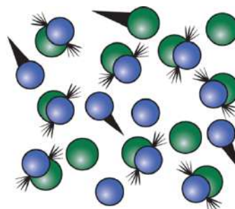
Figure 5.2. Frequency Factor (A) Is Increased by Increasing Concentration
