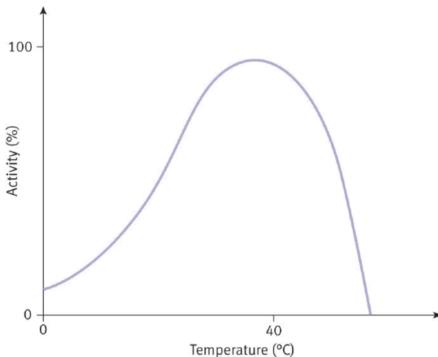
Figure 5.6. An Activity vs. Temperature Curve for a Generic Human Enzyme
