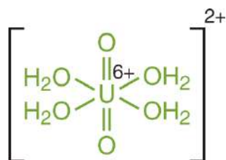
Figure 9.4. Structure of the Tetraaquadioxouranyl Complex Cation Water and oxygen act as ligands with a \text{U}^{6+} cation.
