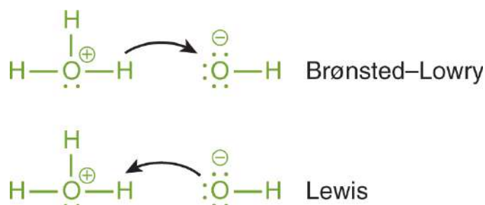
Figure 10.3. Comparison of Brønsted–Lowry and Lewis Definitions of Acids and Bases
