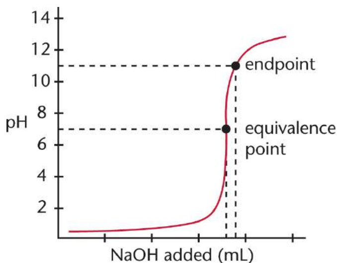
Figure 10.9. Monoprotic Strong Acid and Strong Base Titration Curve A strong base, NaOH, is titrated into a solution of strong acid, HCl, to yield an equivalence point of \text{pH} = 7 .
