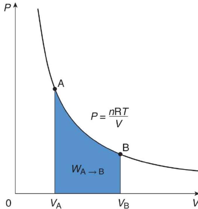
Figure 7.1. Graph of an Isothermal Expansion
