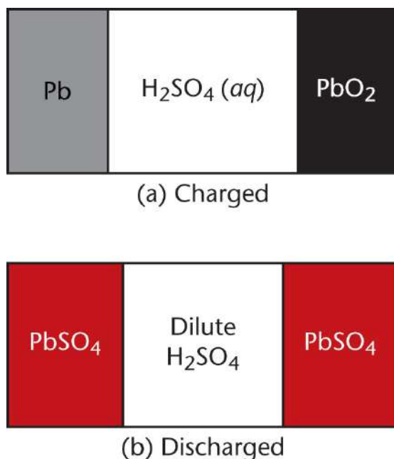
Figure 12.4. Lead–Acid Battery
