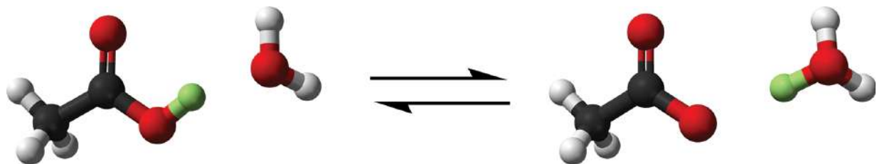
Figure 9.3. Transfer of a Proton in Solution, Forming the Hydronium Ion The transferred proton is highlighted in green.
