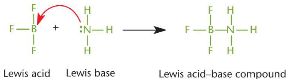
Figure 10.2. Lewis Acid–Base Chemistry
