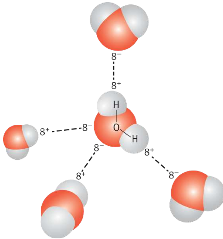
Figure 3.15. Hydrogen Bonding in Water
