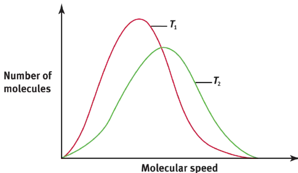
Figure 8.7. Maxwell–Boltzmann Distribution Curves of Molecular Speeds at Two Different Temperatures
