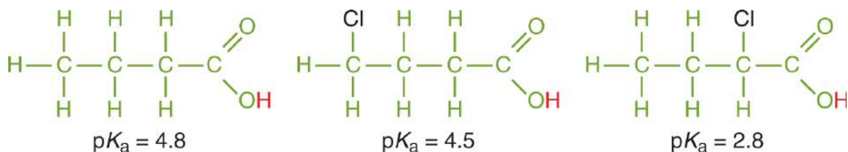
Figure 10.6. Inductive Effects from Electronegative Elements Increase Acidity
