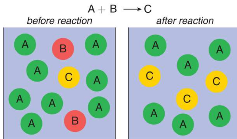
Figure 4.7. Reaction with a Limiting Reagent A is considered an excess reagent; B is the limiting reagent.
