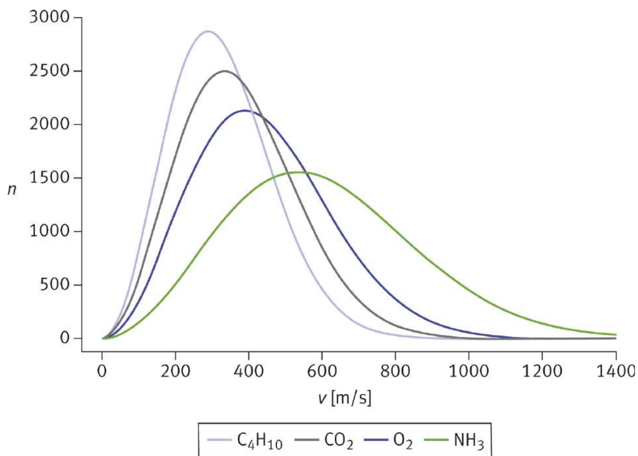
Figure 8.9. Maxwell-Boltzmann Distribution Curves of Molecular Speeds for Gases with Different Molar Masses
