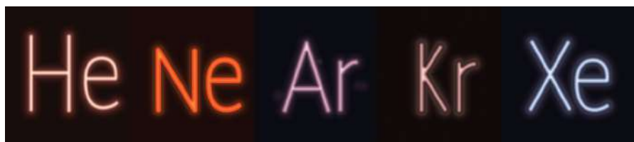
Figure 2.13. Noble Gases Used in “Neon” Signs
