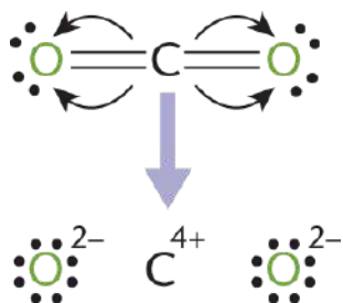
Figure 11.2. Assigning Oxidation Numbers to Carbon Dioxide
