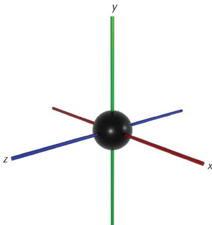
Figure 3.12. 1s -Orbital
