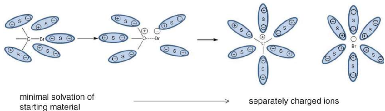
Figure 9.1. Solvation of a Polar Covalent Compound S indicates a solvent particle.
