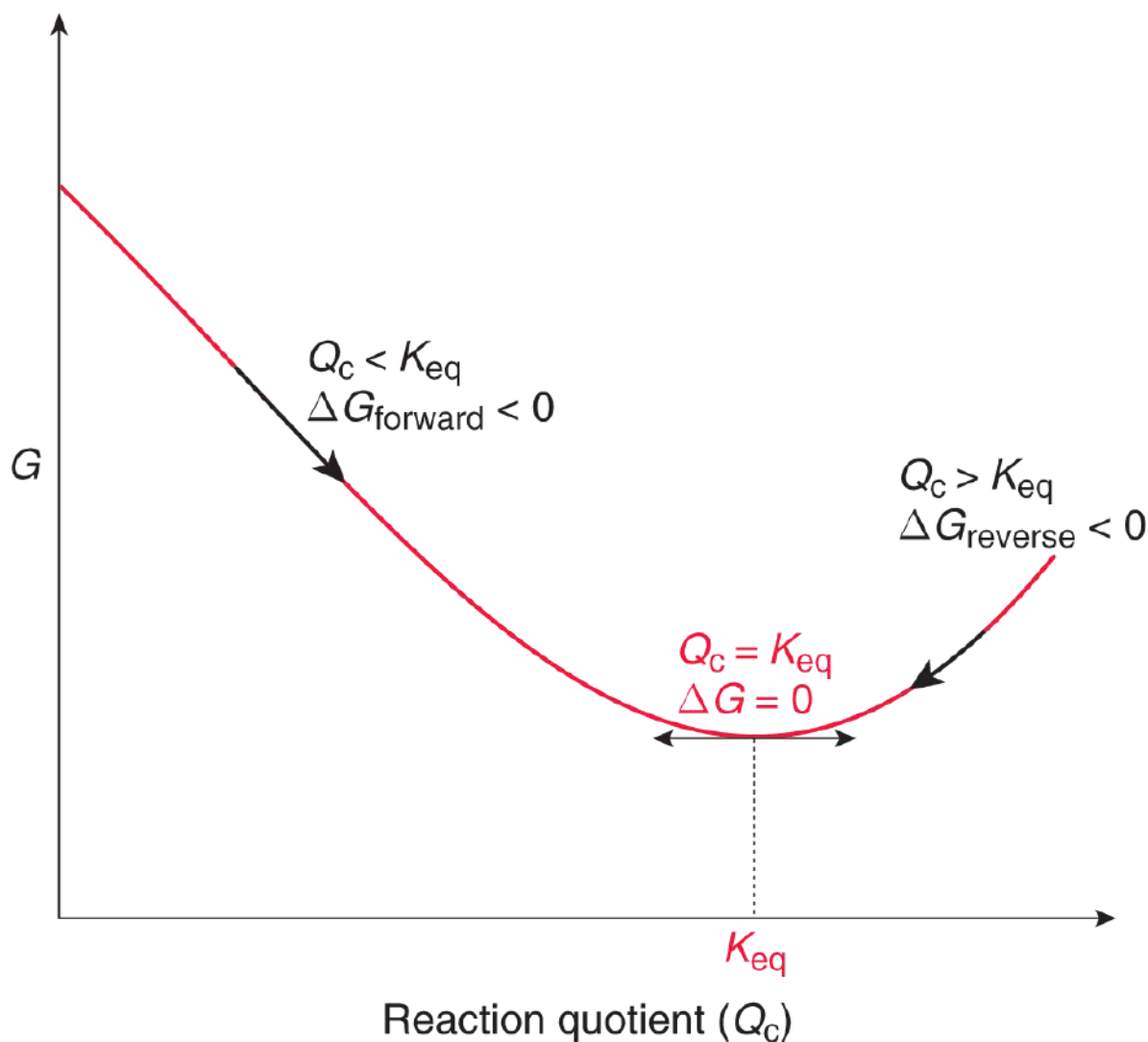
Figure 7.11. Gibbs Free Energy and Spontaneity
