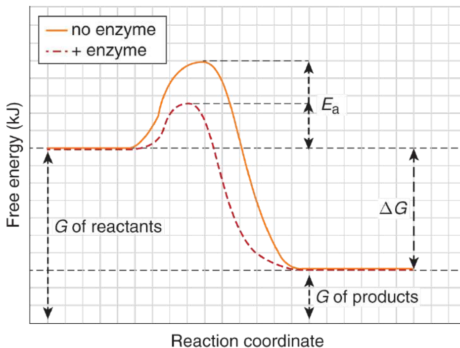
Figure 7.14. Catalysts Alter Kinetics but Not Equilibrium or Free Energy Change
