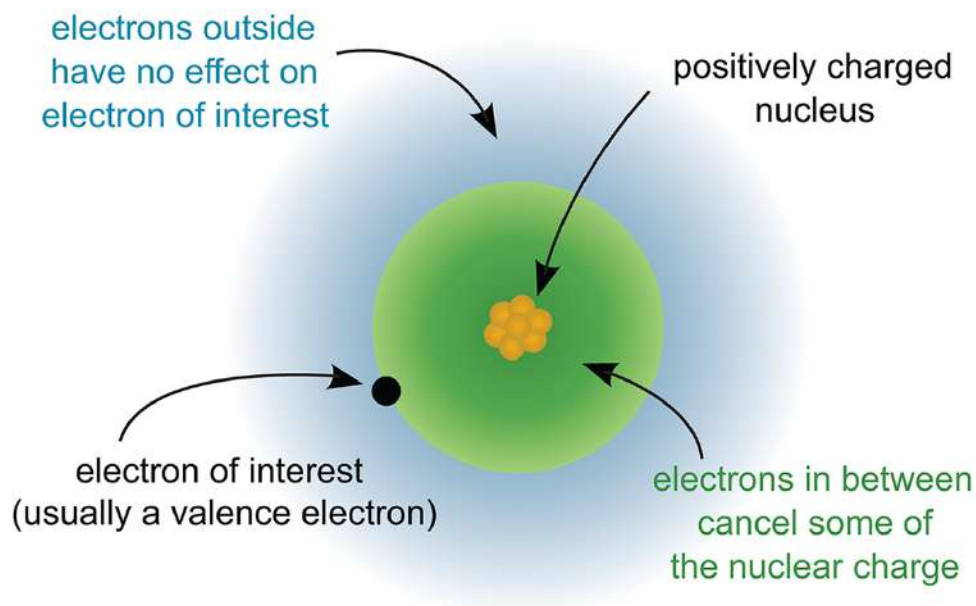
Figure 2.4. Factors that Determine Effective Nuclear Charge ( Z_{\text{eff}} )
