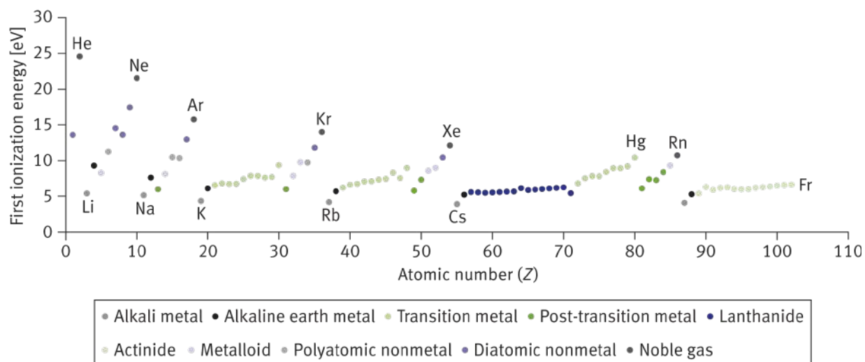
Figure 2.7. First Ionization Energies (in eV) of the Elements
