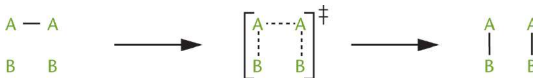
Figure 5.3. The Transition State
