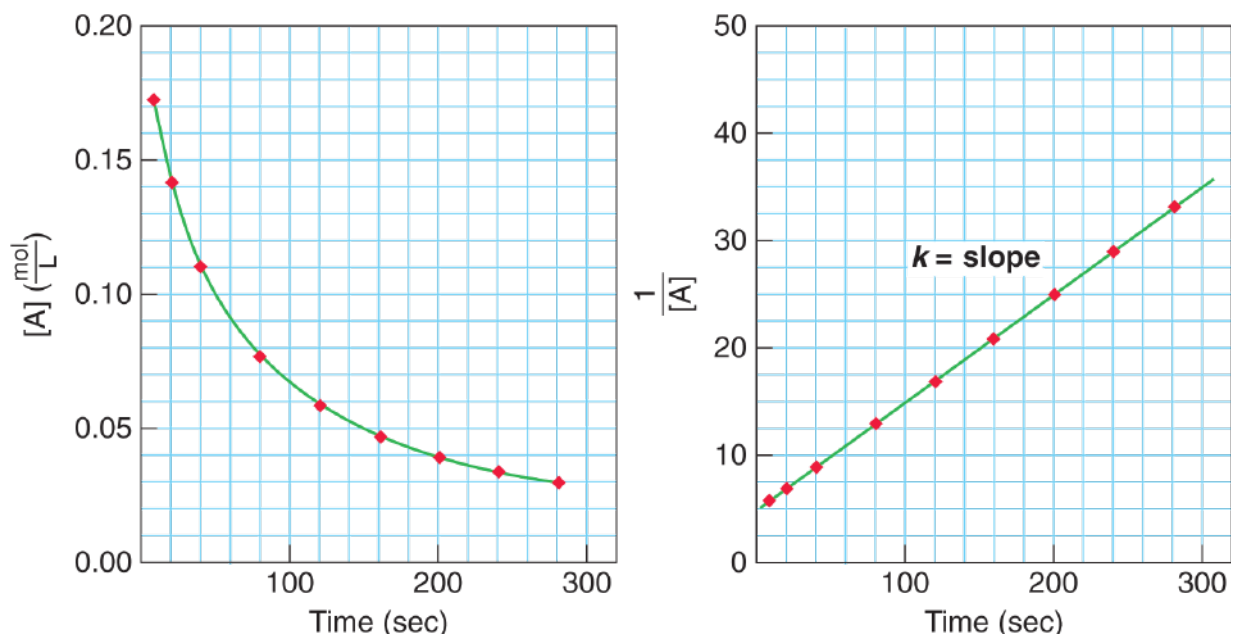
Figure 5.10. Kinetics of a Second-Order Reaction
