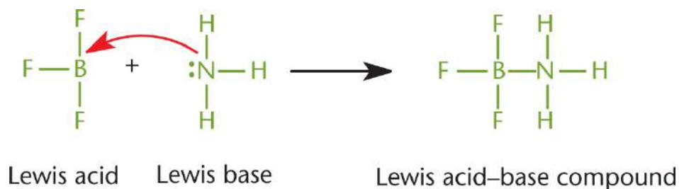
Figure 3.7. Coordinate Covalent Bond
