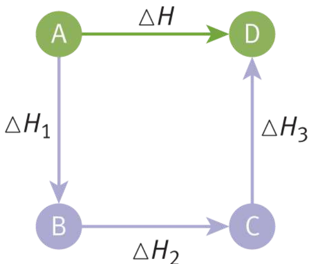
Figure 7.8. Illustration of Hess's Law: Forming Product (D) from Reactant (A)
