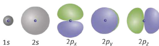
Figure 1.11. The First Five Atomic Orbitals
