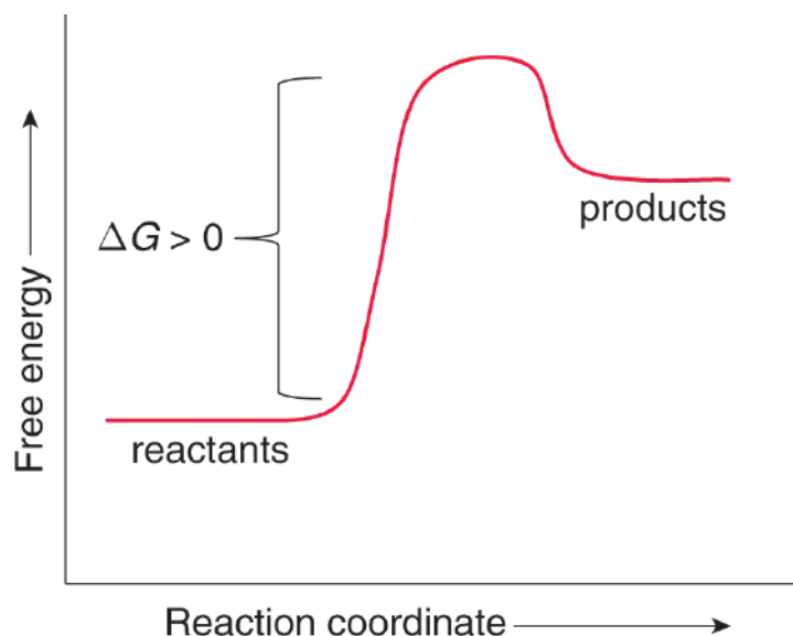
Figure 7.13. Endergonic Reaction Profile
