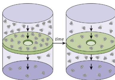
Figure 8.10. Effusion of Gas Particles
