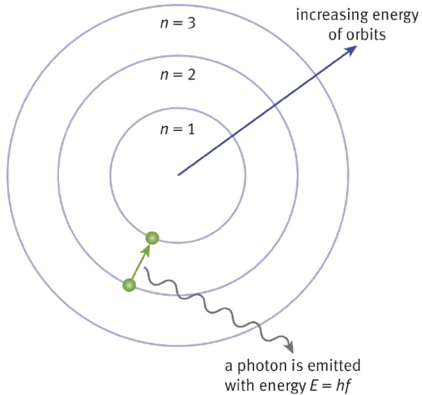
Figure 1.5. Atomic Emission of a Photon as a Result of a Ground State Transition
