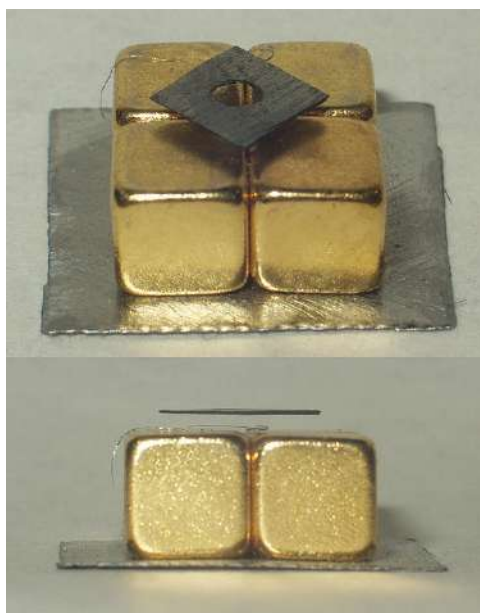
Figure 1.15. Diamagnetic Pyrolytic Graphite
