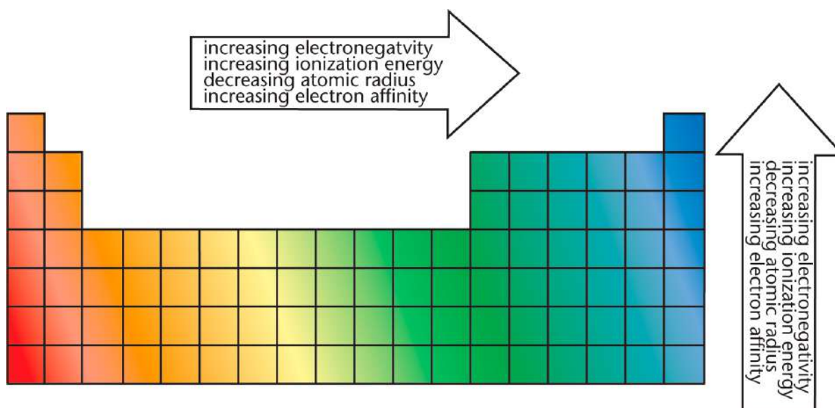
Figure 2.10. Periodic Trends
