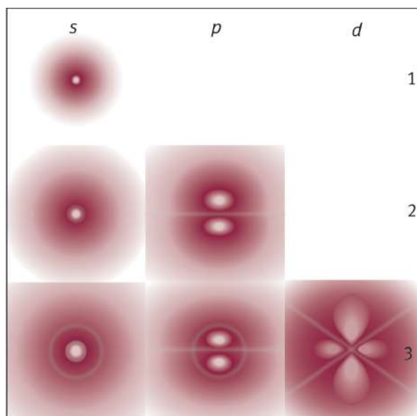
Figure 1.10. Electron Clouds of Various Subshells
