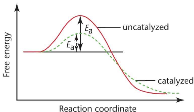
Figure 5.7. Reaction Diagram for a Catalyzed and an Uncatalyzed Reaction
