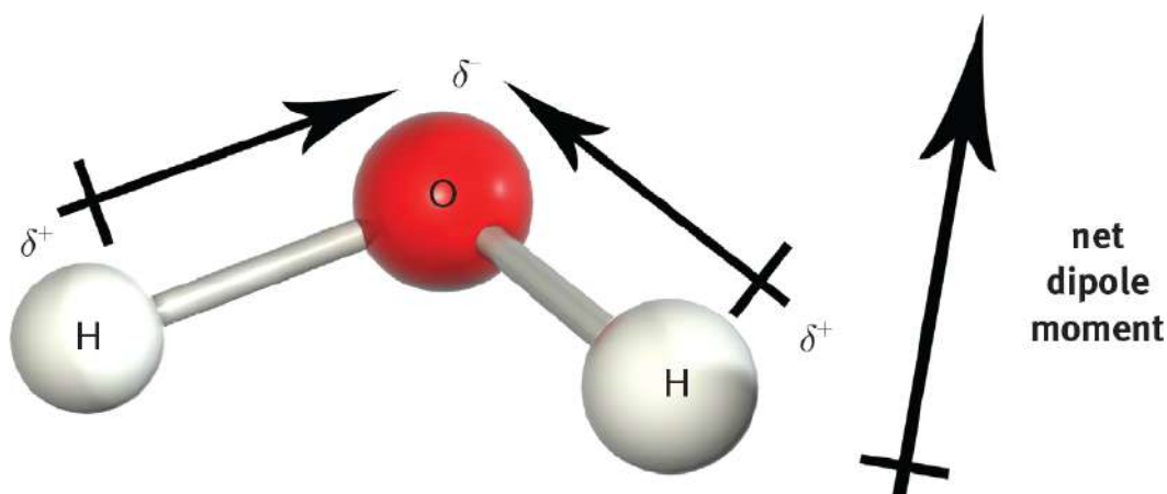
Figure 3.11. \text{H}_2\text{O} is a Polar Molecule with Two Polar Bonds
