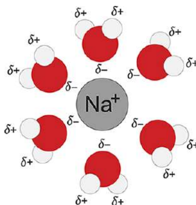
Figure 9.2. Solvation of \text{Na}^+ Ions in Aqueous Solutions
