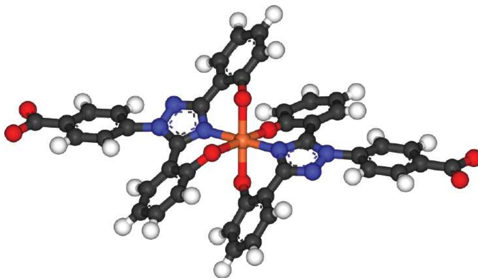
Figure 9.8. Chelation of Iron with Two Molecules of Deferasirox
