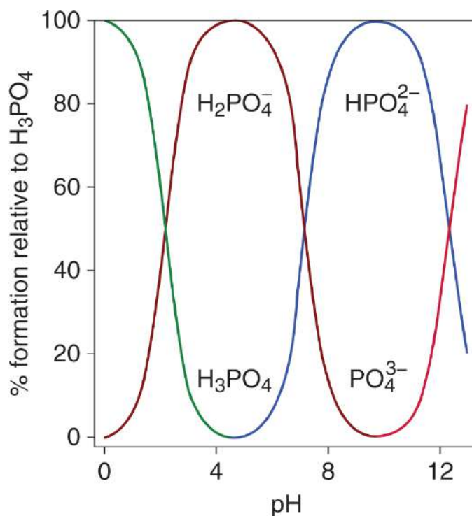
Figure 10.8. Speciation Plot of Phosphoric Acid
