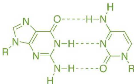
Figure 3.16. Hydrogen Bonding between Guanine and Cytosine
