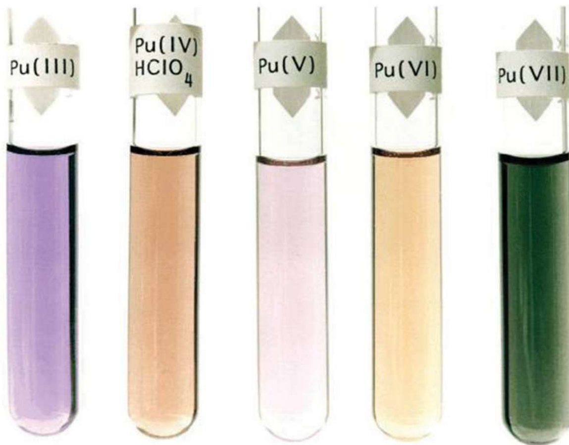
Figure 4.9. Solutions with Various Plutonium Oxidation States
