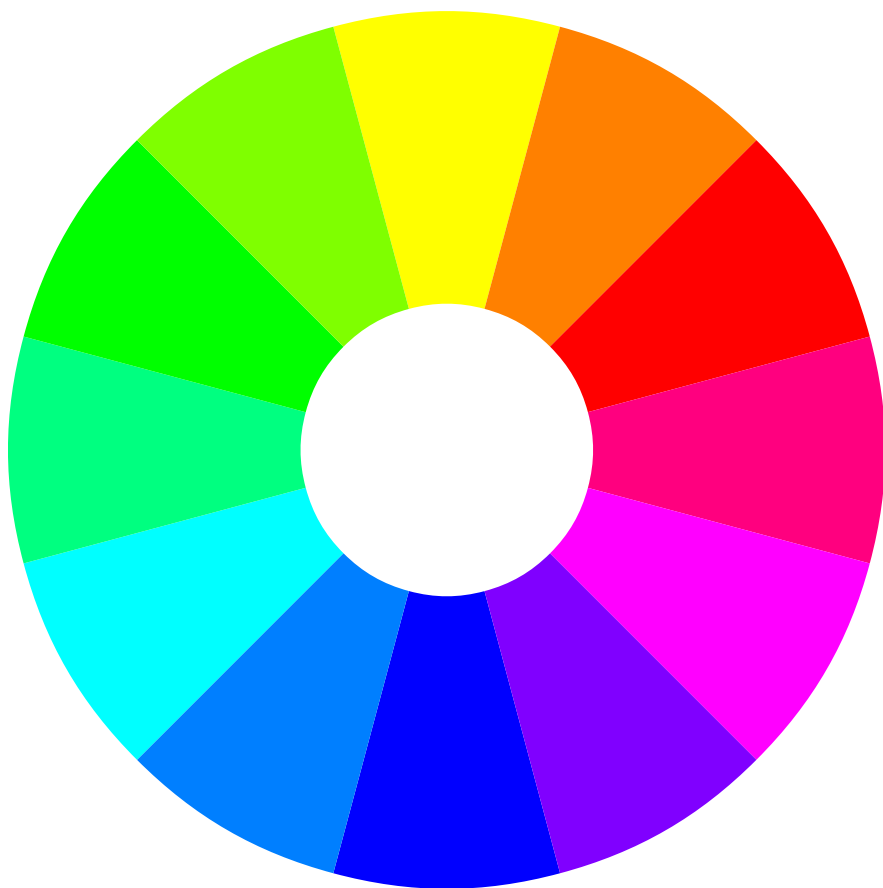
Figure 2.15. Red–Green–Blue (Additive) Color Wheel
