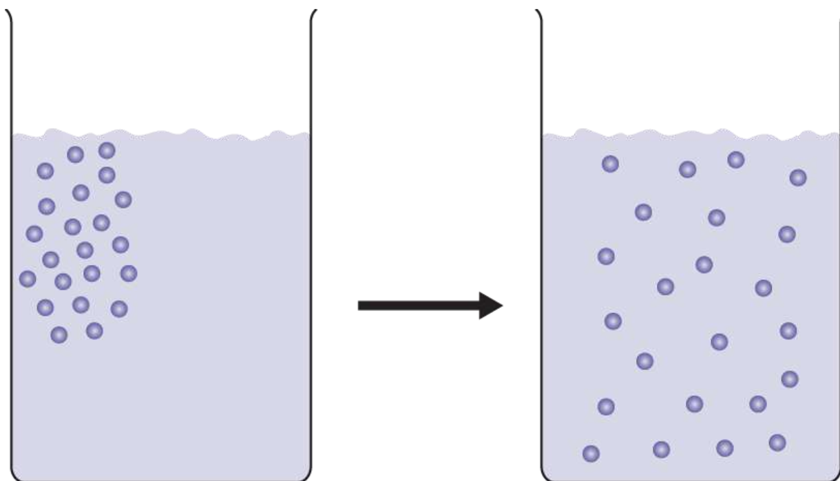
Figure 8.8. Diffusion of Solutes in a Solvent
