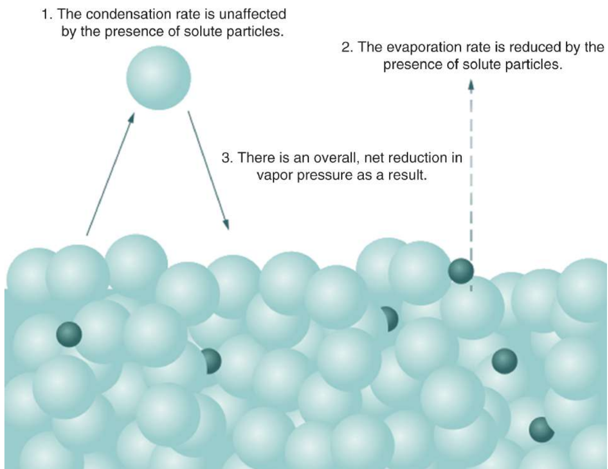
Figure 9.10. Molecular Basis of Raoult's Law
