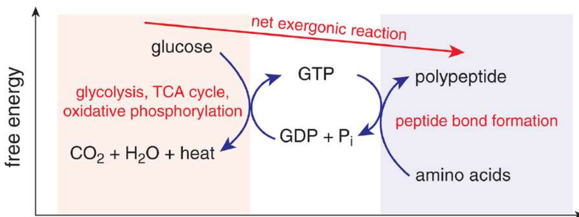
Figure 7.4. Coupling of Reactions
