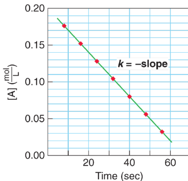
Figure 5.8. Kinetics of a Zero-Order Reaction
