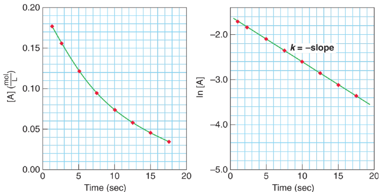
Figure 5.9. Kinetics of a First-Order Reaction
