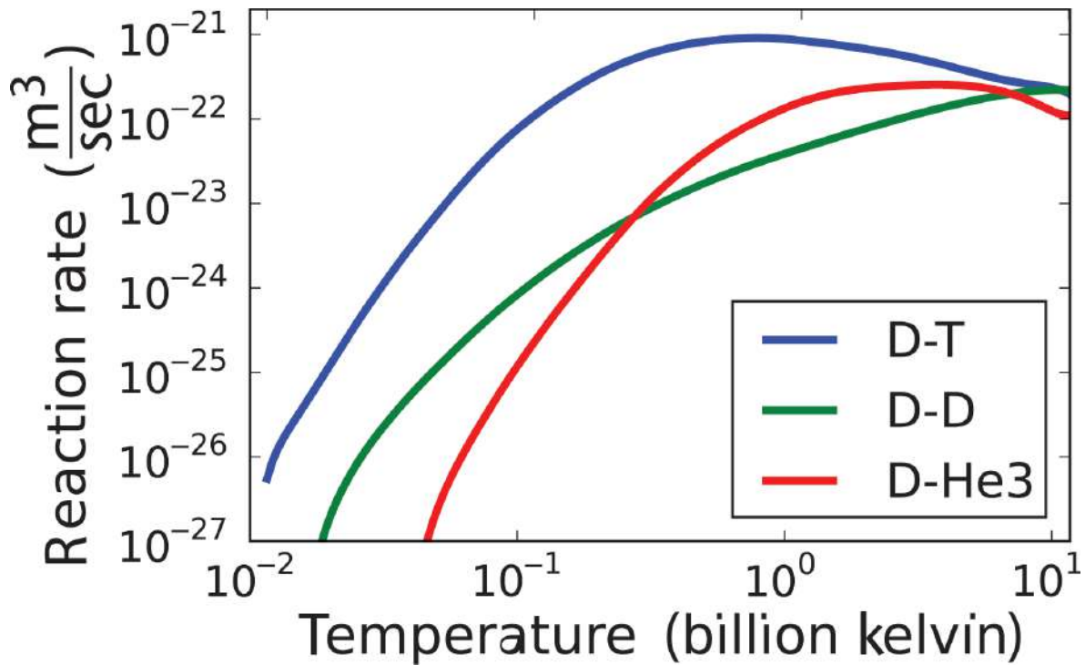
Figure 5.5. All Reactions Are Temperature-Dependent
