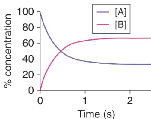
Figure 6.1. Dynamic Equilibrium Occurs when Forward and Reverse Rates Are Equal
