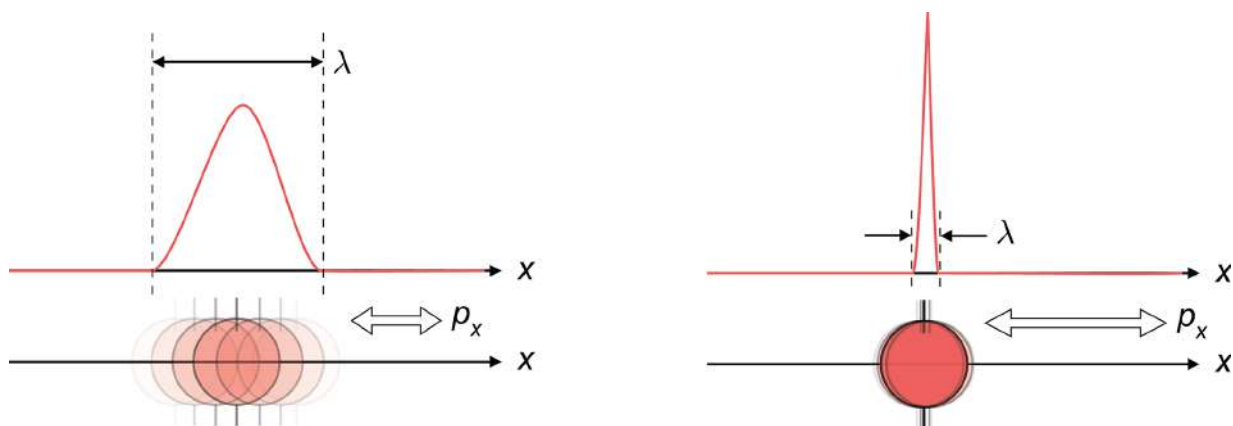
Figure 1.8. Heisenberg Uncertainty Principle
