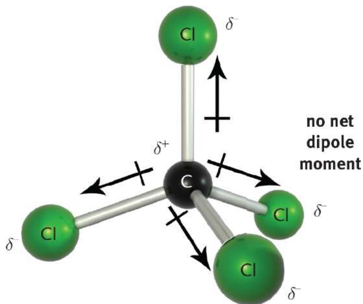
Figure 3.10. \text{CCl}_4 is a Nonpolar Compound with Four Polar Bonds
