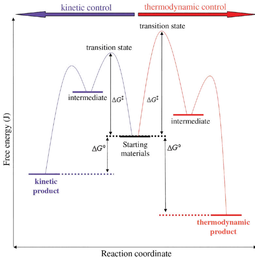
Figure 6.4. Kinetic and Thermodynamic Control of a Reaction
