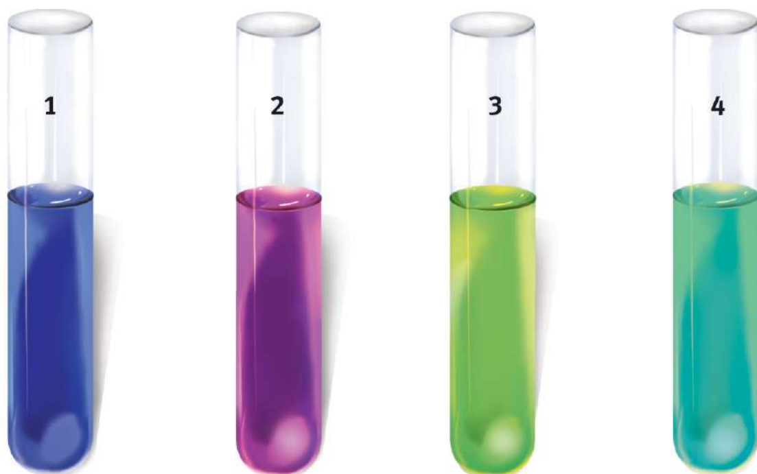
Figure 9.7. Nickel(II) Ion Complexes Display Distinctive Colors
