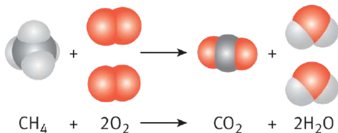
Figure 4.4. Combustion of Methane
