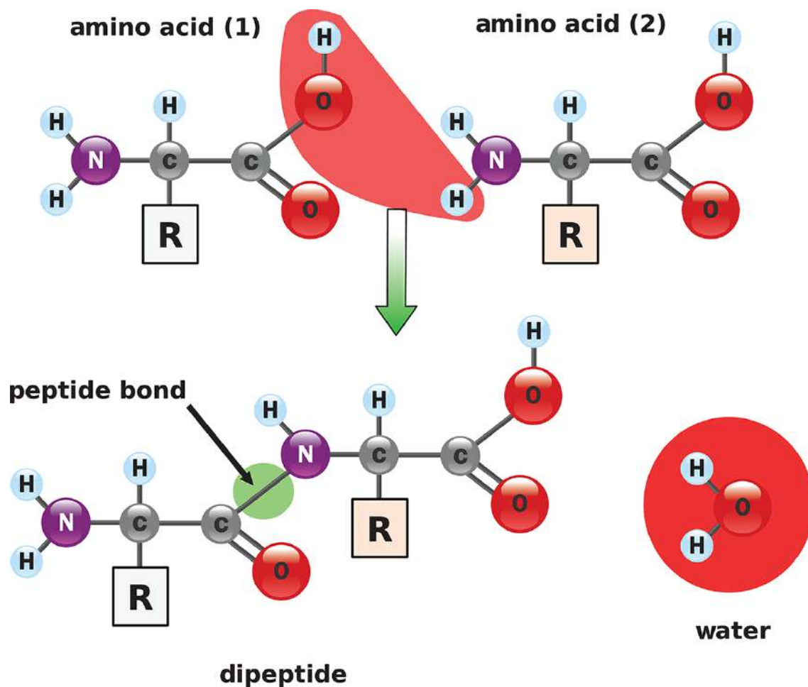
Figure 10.7. Peptide Bond Formation
