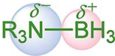
Figure 3.5. Polar Covalent Bond in an Amine Borane
