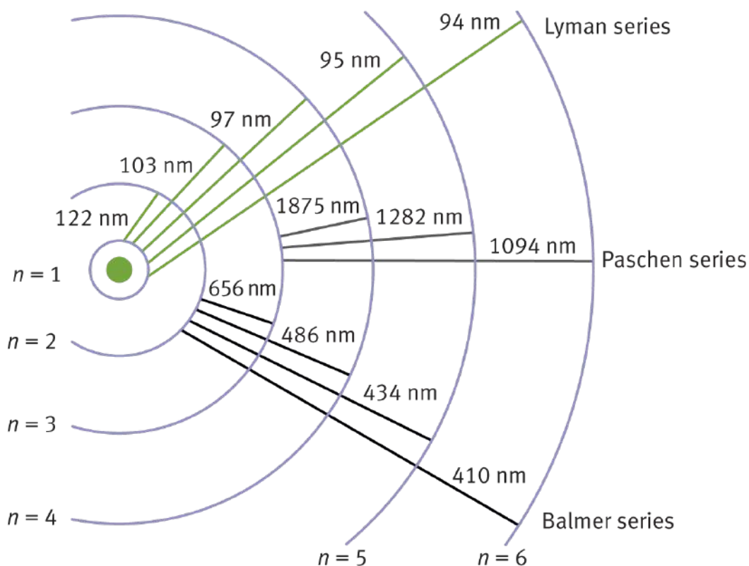
Figure 1.7. Wavelengths of Electron Orbital Transitions
