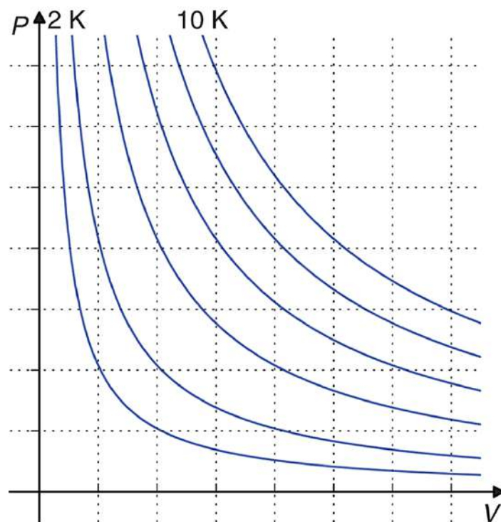
Figure 8.2. Ideal Gas Isothermal Curves
