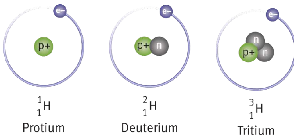
Figure 1.3. Various Isotopes of Hydrogen
