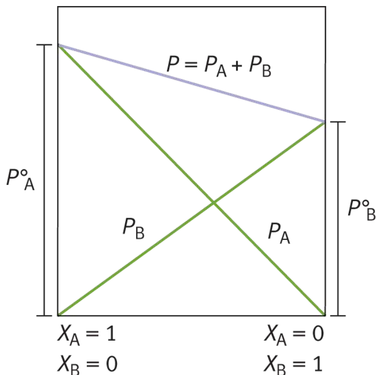
Figure 9.9. Raoult's Law
