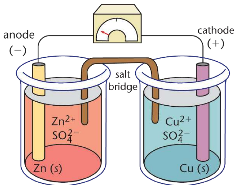
Figure 12.1. Daniell Cell
