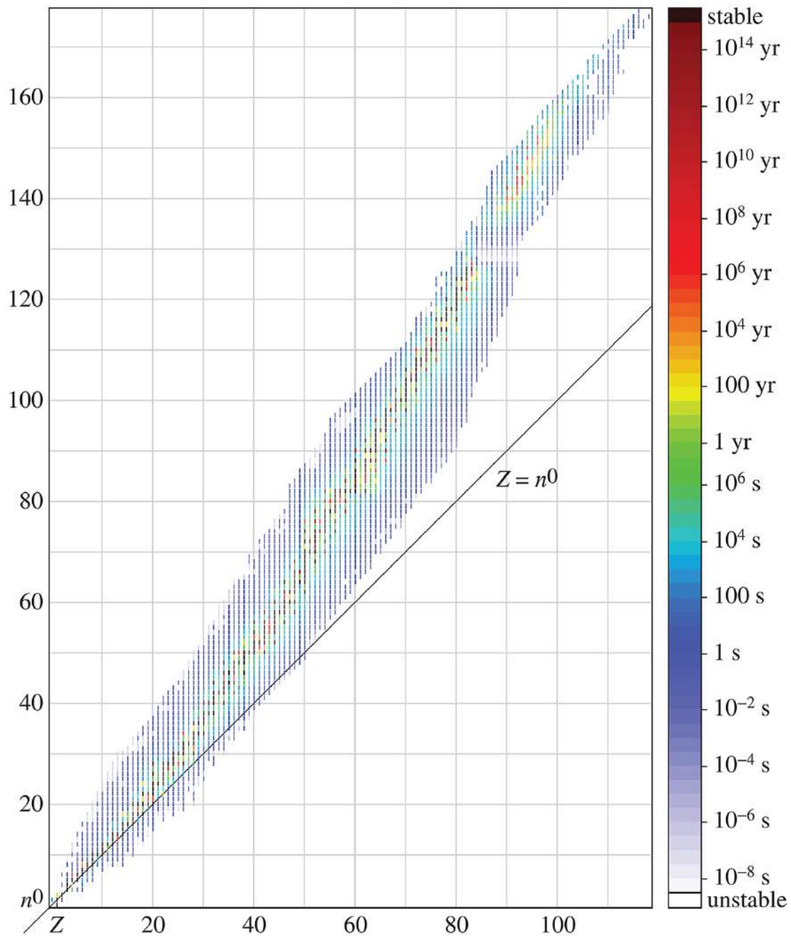
Figure 1.4. Half-Lives of the Different Isotopes of Elements Half-life is a marker of stability; generally, longer-lasting isotopes are more abundant.
