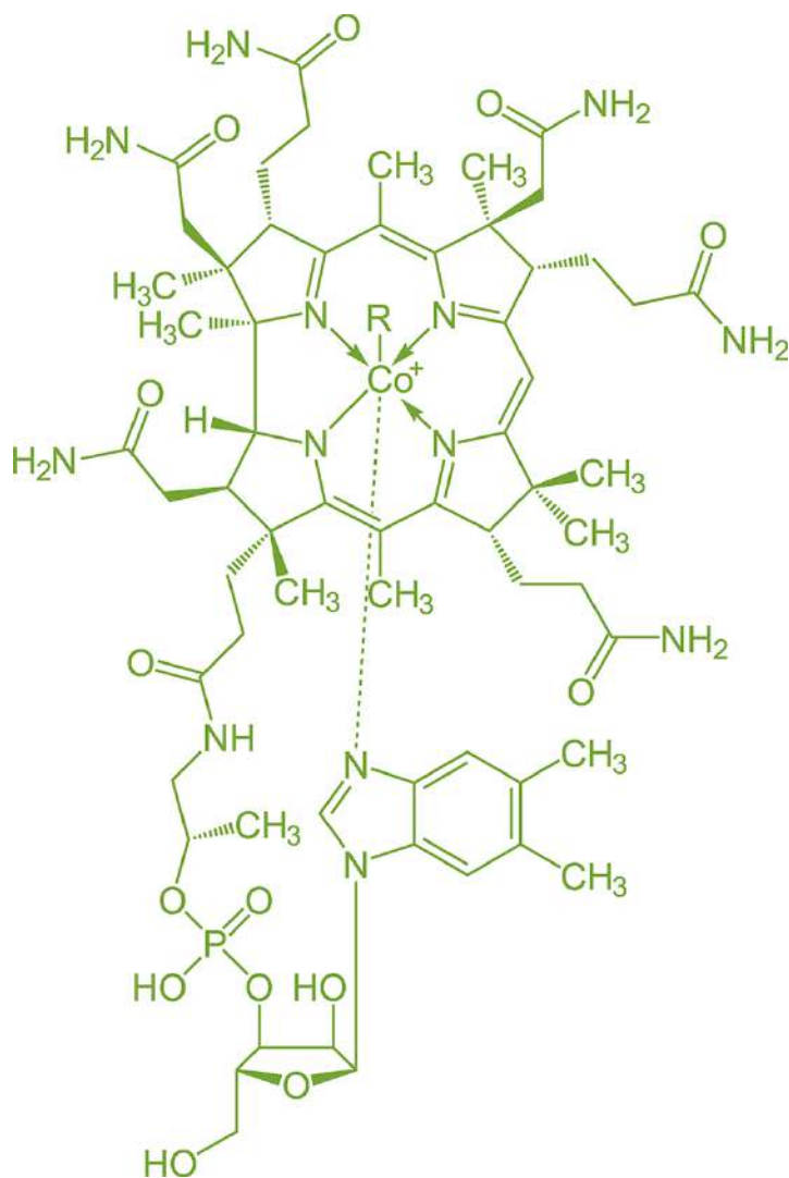
Figure 9.6. Cobalamin (Vitamin B 12 ) Contains a Cobalt Complex
