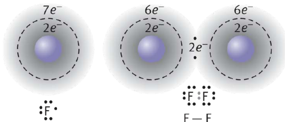
Figure 3.4. Formation of a Covalent Bond
