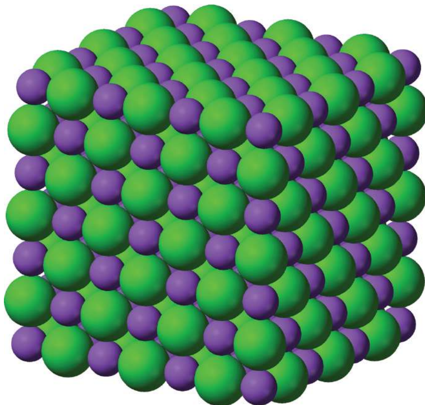
Figure 3.3. Crystal Lattice Structure of Sodium Chloride Sodium = purple; chloride = green
