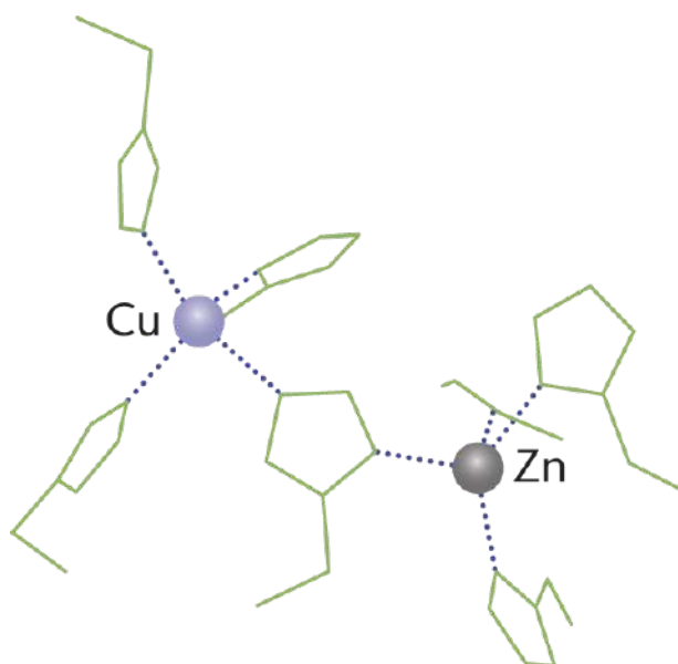
Figure 11.3. Active Site of Superoxide Dismutase
