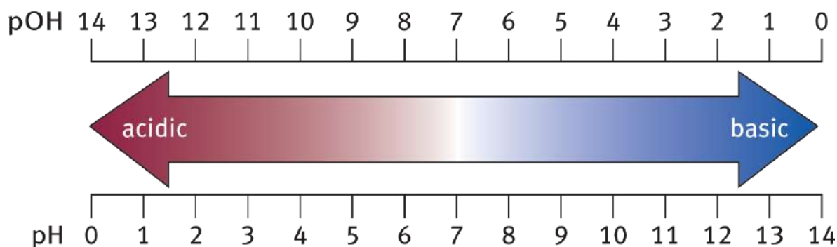
Figure 10.5. pH and pOH Scales
