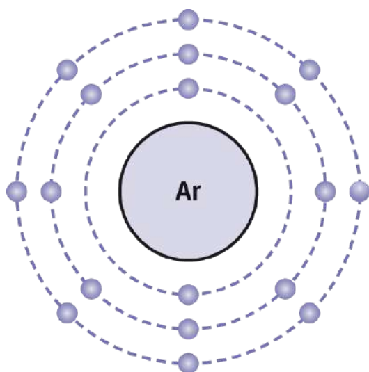
Figure 3.1. Electron Configuration of Argon As a noble gas, argon has a complete octet in its valence shell.
