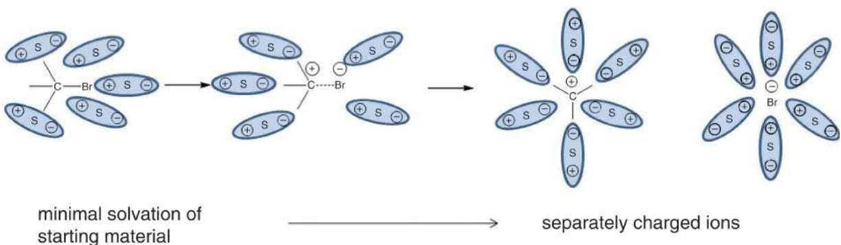
Figure 4.10. Solvation of a Polar Covalent Compound S indicates a solvent particle.
