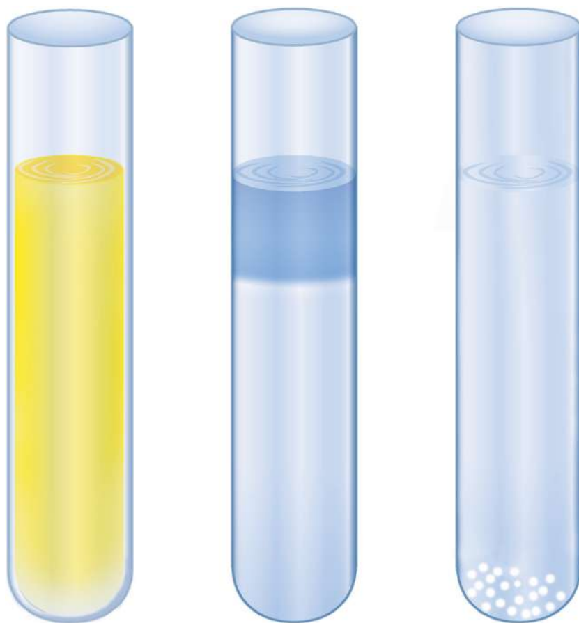
Figure 4.5. Illustrations of Double-Displacement Reactions Forming Zinc Salts
