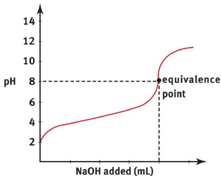
Figure 10.10. Weak Acid and Strong Base Titration Curve
