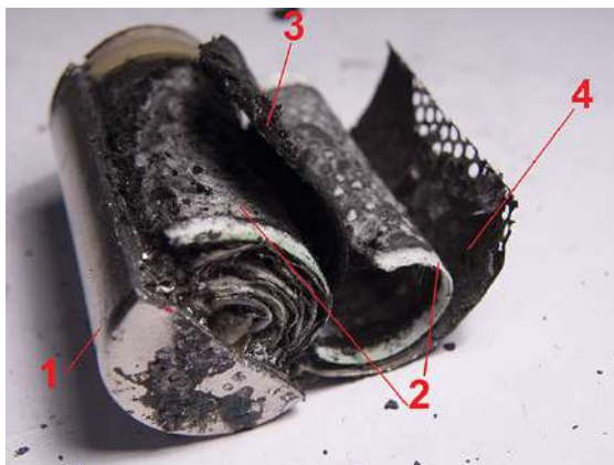
Figure 12.5. A Nickel–Cadmium Battery
