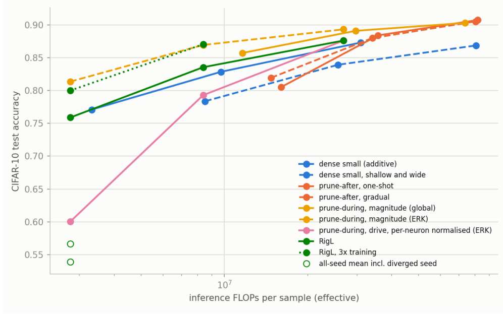
Figure 2: CIFAR-10 accuracy against inference FLOPs; each point is one budget. At equal FLOPs, prune-during with the ERK allocation (yellow, dashed) dominates RigL (dark green) and the dense small network (blue). RigL at 1% is plotted as the mean of the two seeds that converged (75.9%), as in Table 2; the hollow markers are three-seed means that include a diverged seed (53.9% for RigL, 56.7% for RigL at 3\times training length).
