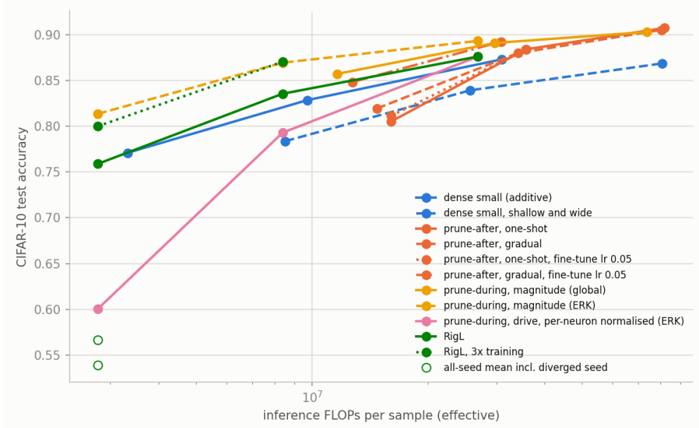
Figure 2: CIFAR-10 accuracy against inference FLOPs; each point is one budget. At equal FLOPs and equal training length, prune-during with the ERK allocation (yellow, dashed) dominates RigL (dark green) and the dense small network (blue); RigL trained three times longer (dark green, dotted) reaches the ERK line at 3%. Orange: prune-after, one-shot (solid) and gradual (dashed) at the standard fine-tuning rate and both at the training rate (dotted, dash-dotted); blue dashed: the shallow-and-wide dense small network. RigL at 1% is plotted as the mean of the two seeds that converged (75.9%), as in Table 2; the hollow markers are three-seed means that include a diverged seed (53.9% for RigL, 56.7% for RigL at 3\times training length).
