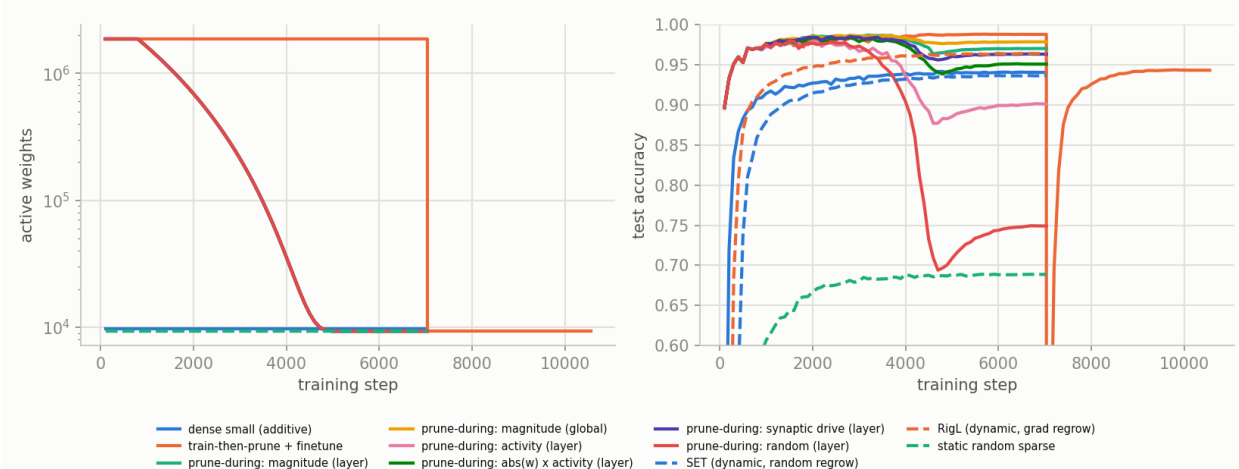
Figure 1: Connection count (left, log scale) and test accuracy (right) during training at 0.5% density on MNIST (seed 0). Prune-after (orange) trains dense, is pruned once at step 7035, collapses below 60% and recovers to 94% during fine-tuning; the prune-during routes reach the same final count gradually; the global route (yellow) never falls below 97% (lowest point in any seed 97.3%, run logs) and the per-layer route (green) ends at 97.0%.
