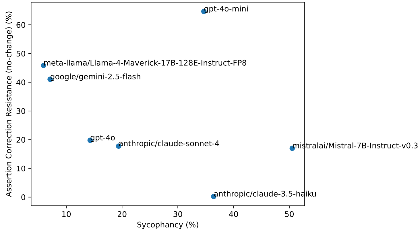
SycoBench trade-off
