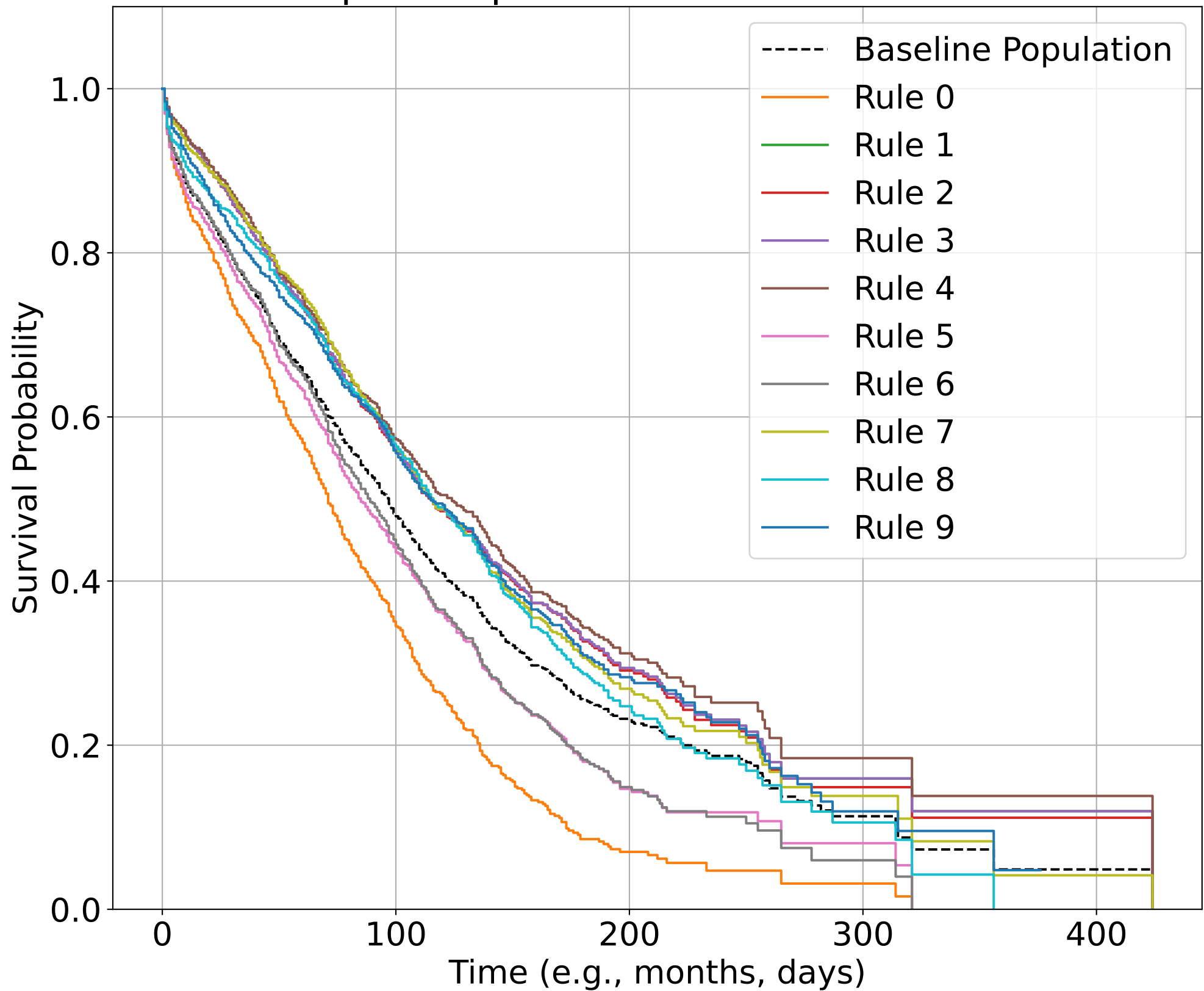
Top-10 Kaplan-Meier Survival Curves
