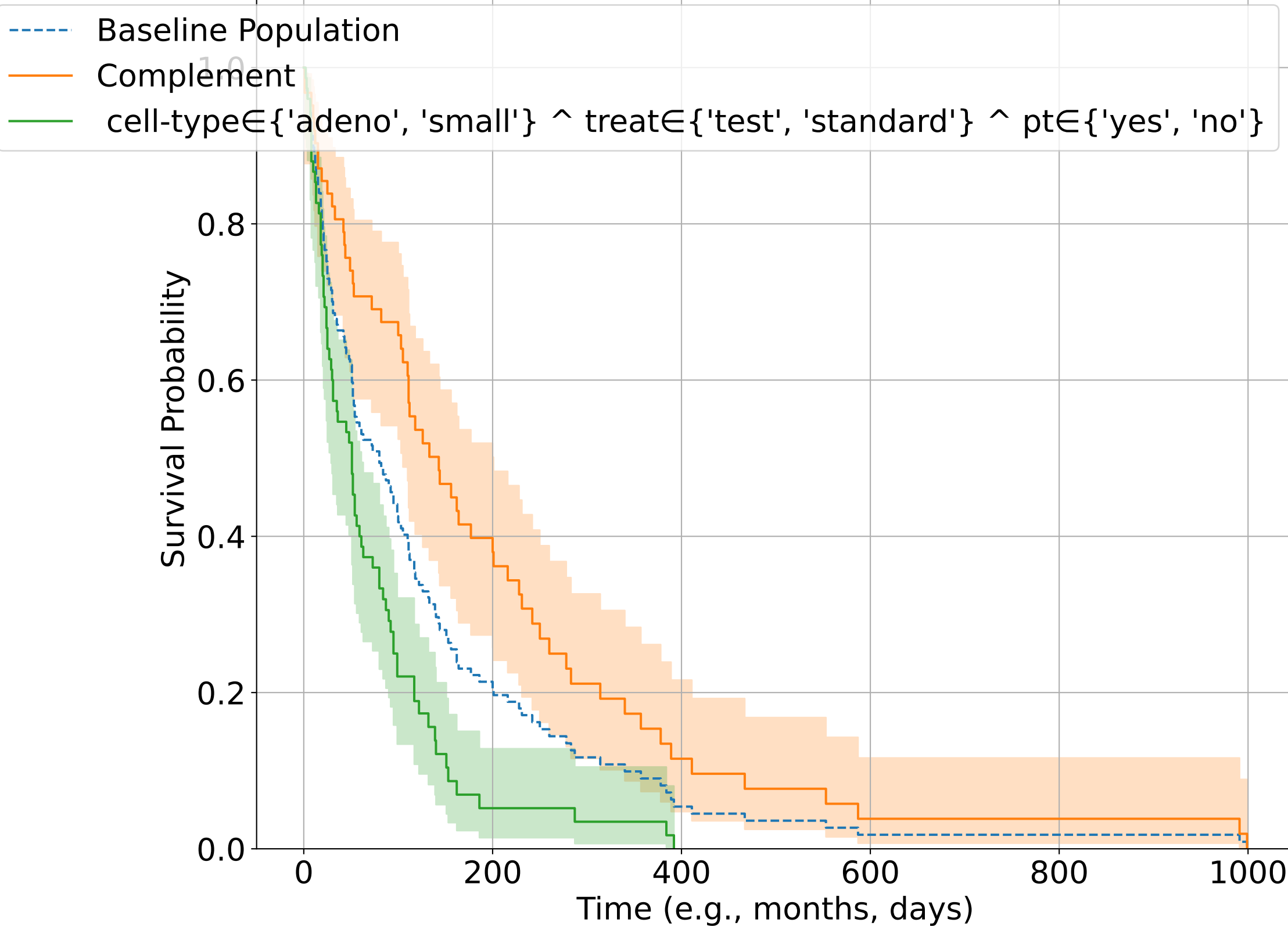
Top-1 Kaplan-Meier Survival Curves
