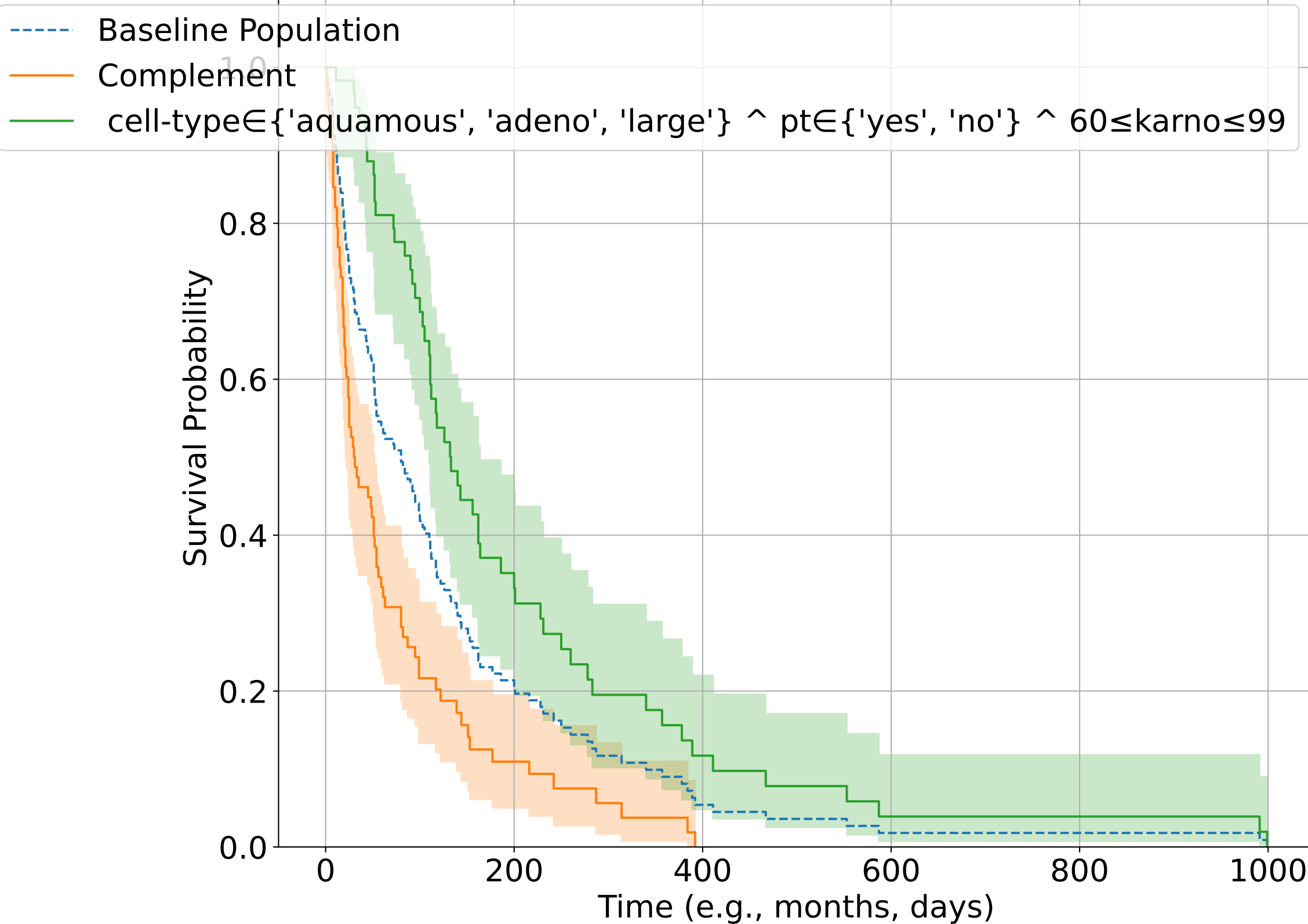
Top-9 Kaplan-Meier Survival Curves
