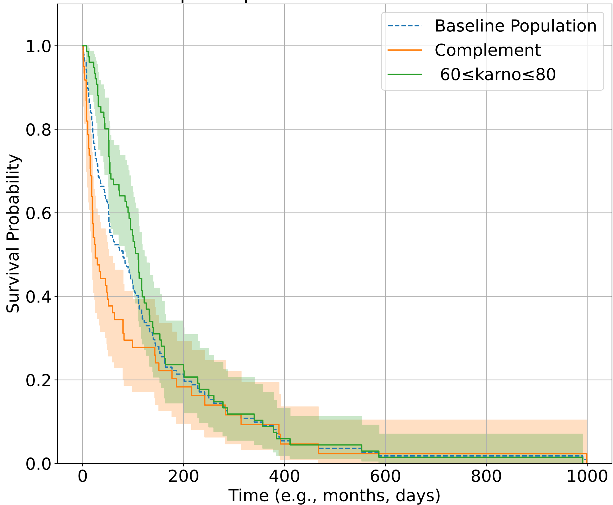
Top-9 Kaplan-Meier Survival Curves
