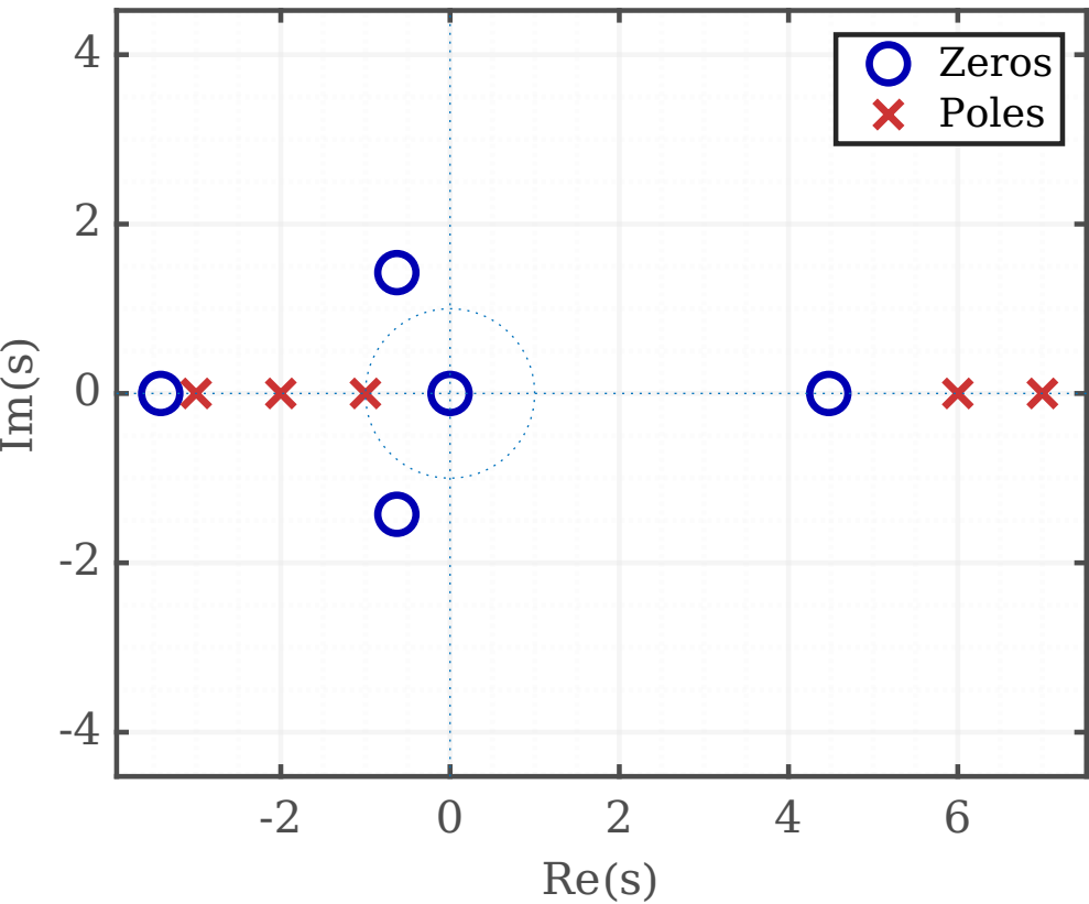
Pole-Zero Plot
