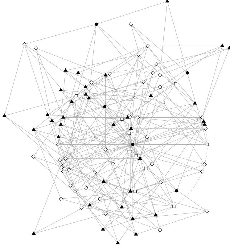
FIGURE 1. The graph over \mathbb{Q}(\sqrt{11}) : 94 points, joined by the 214 segments of length exactly 1 (drawn from the coordinates rounded to five decimals; make_figure.py writes the drawing from the data). The marker shapes show a proper 4-colouring; there is no proper 3-colouring. The vertex at the origin has 32 neighbours, on the dashed unit circle.
