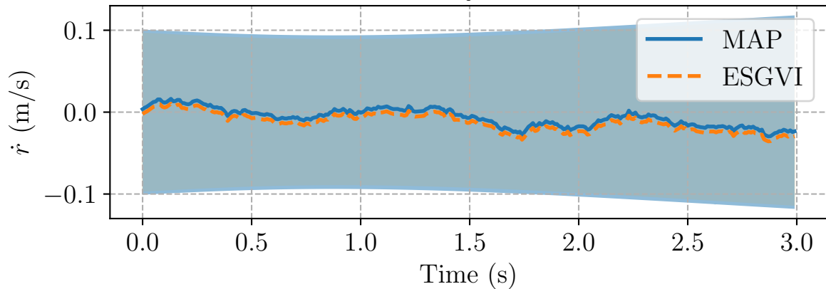
Velocity Error
