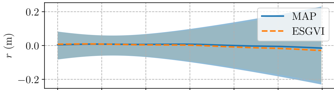
Position Error
