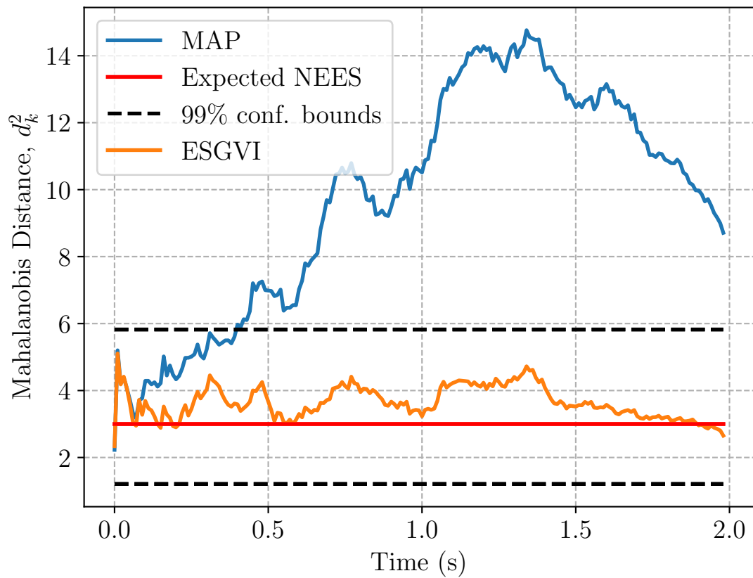
aNEES 10 trials for 3 landmarks.
