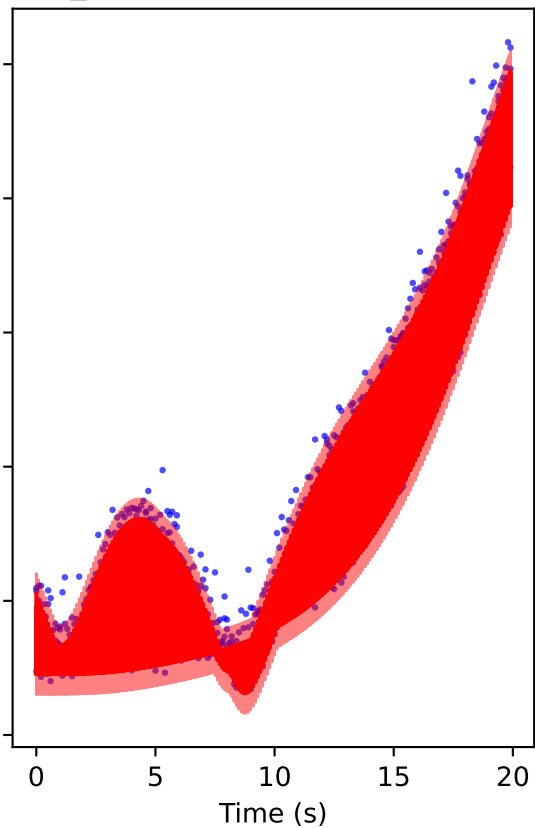
Gaussian Range Measurements Skew_laplace Range Measurements
