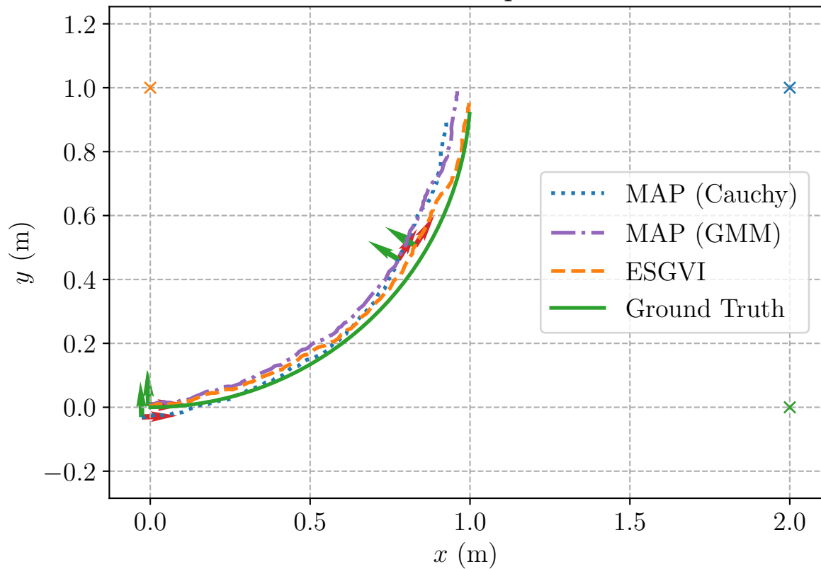
Estimated poses
