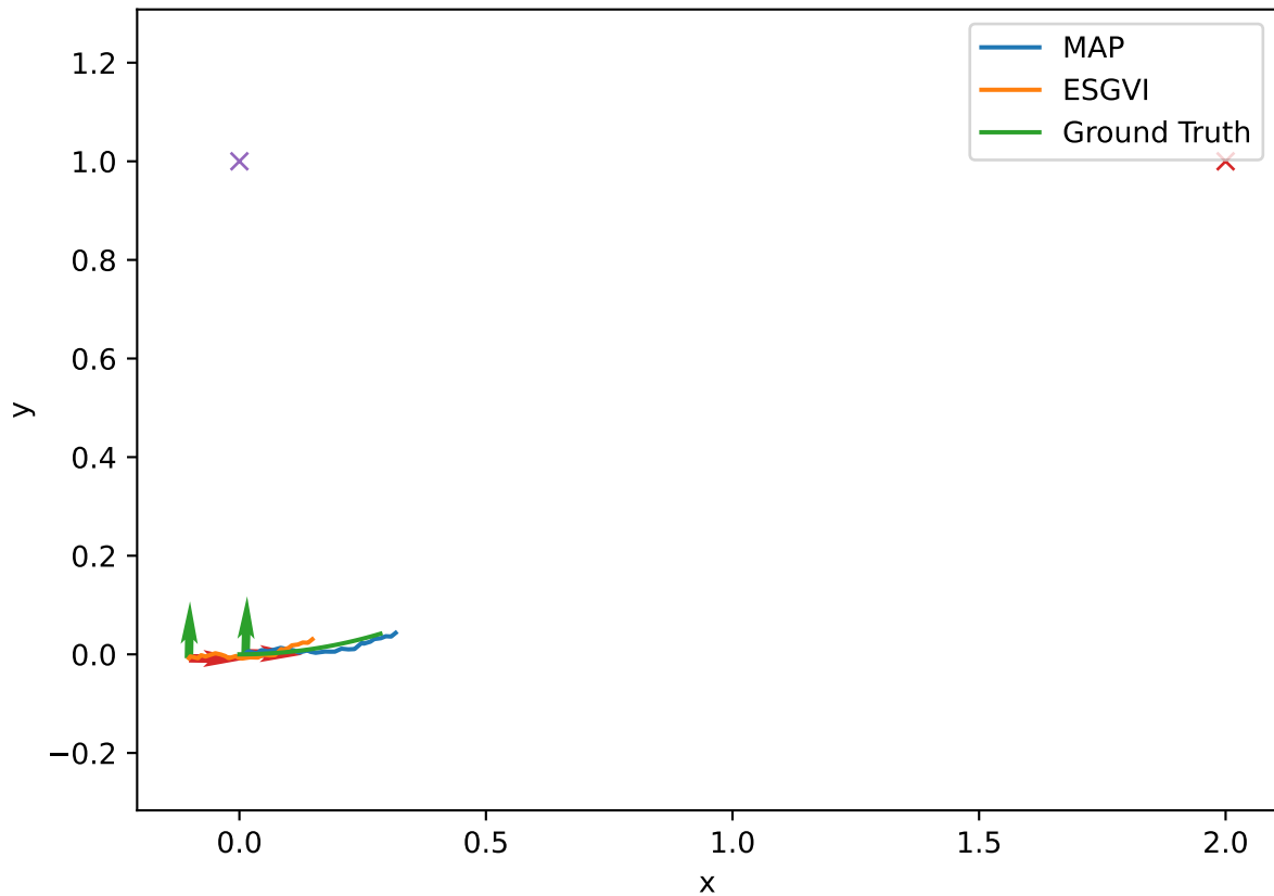
Estimated poses
