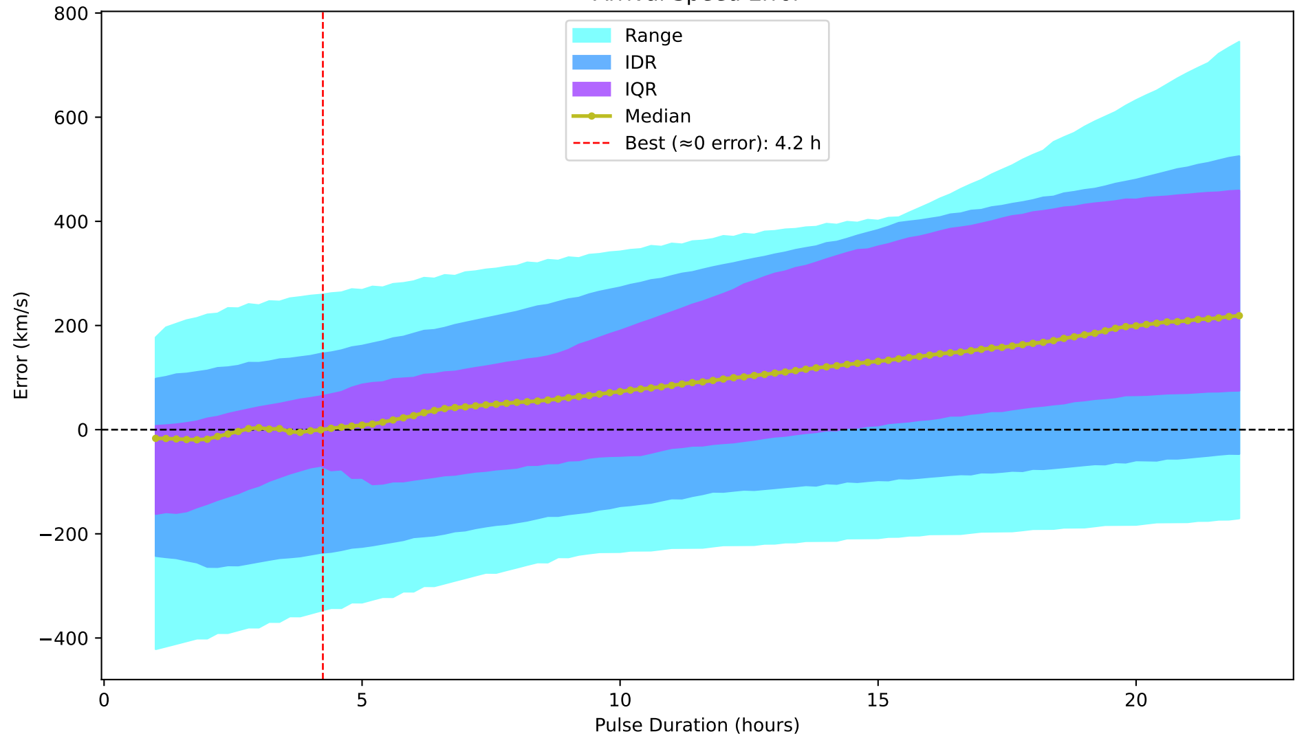
Arrival Speed Error
