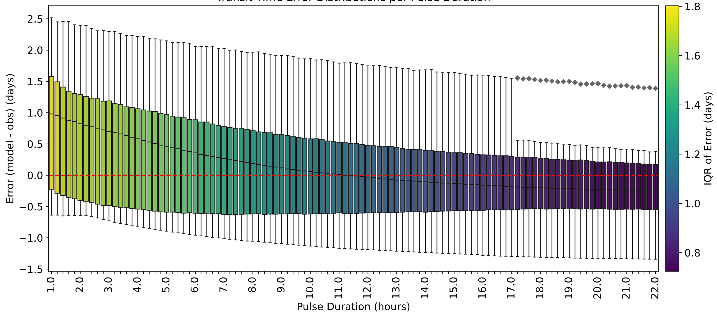
Transit Time Error Distributions per Pulse Duration
