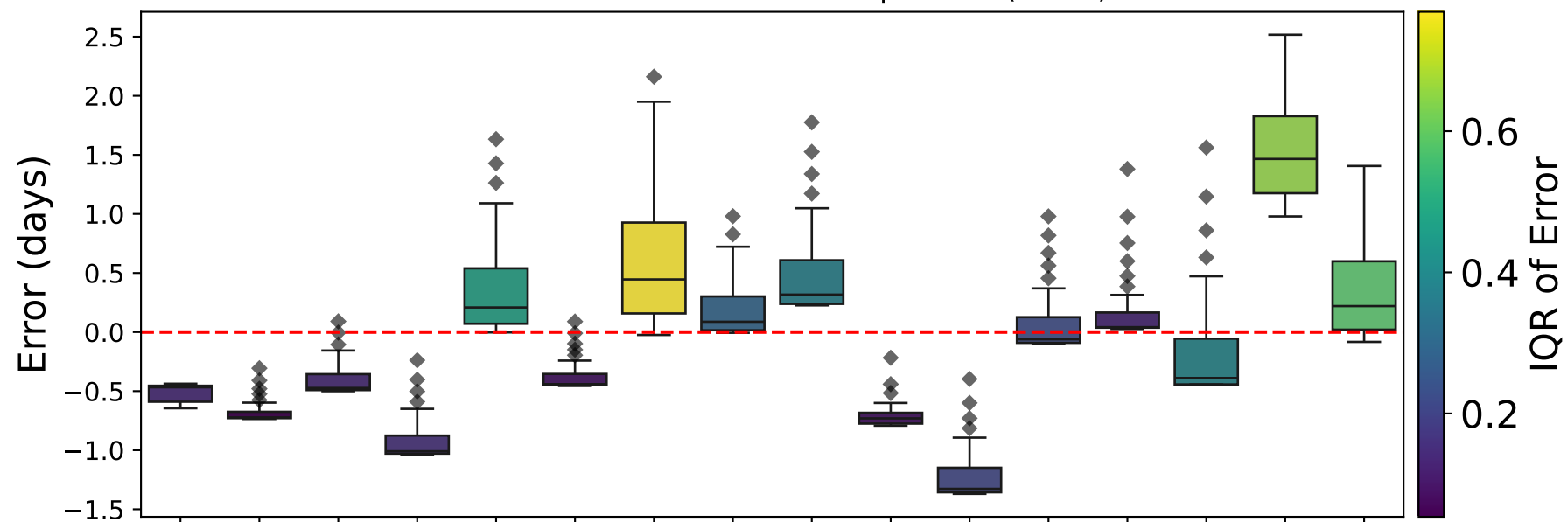
Transit Time Error Distributions per CME (Width)
