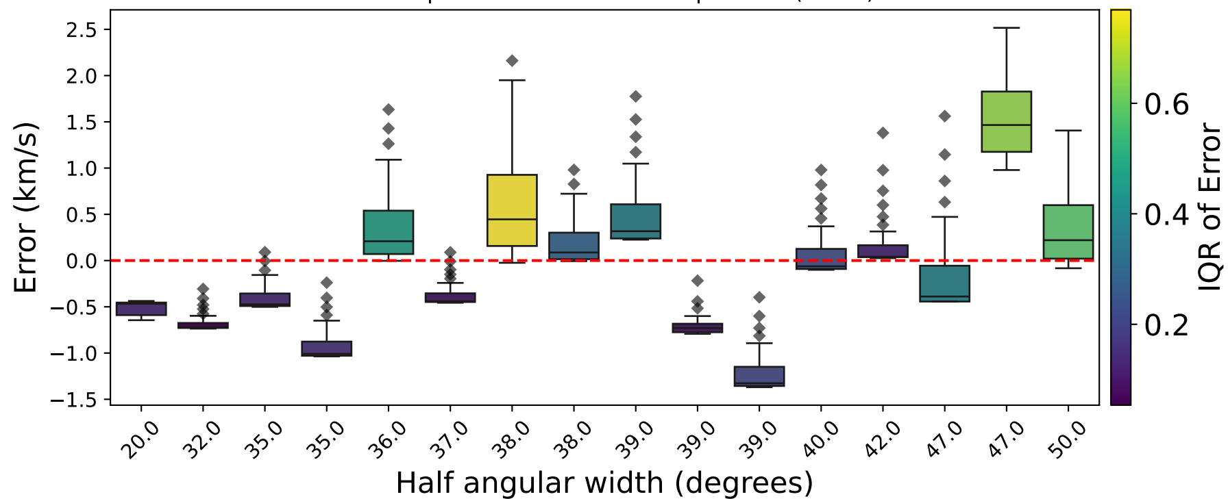
Arrival Speed Error Distributions per CME (Width)
