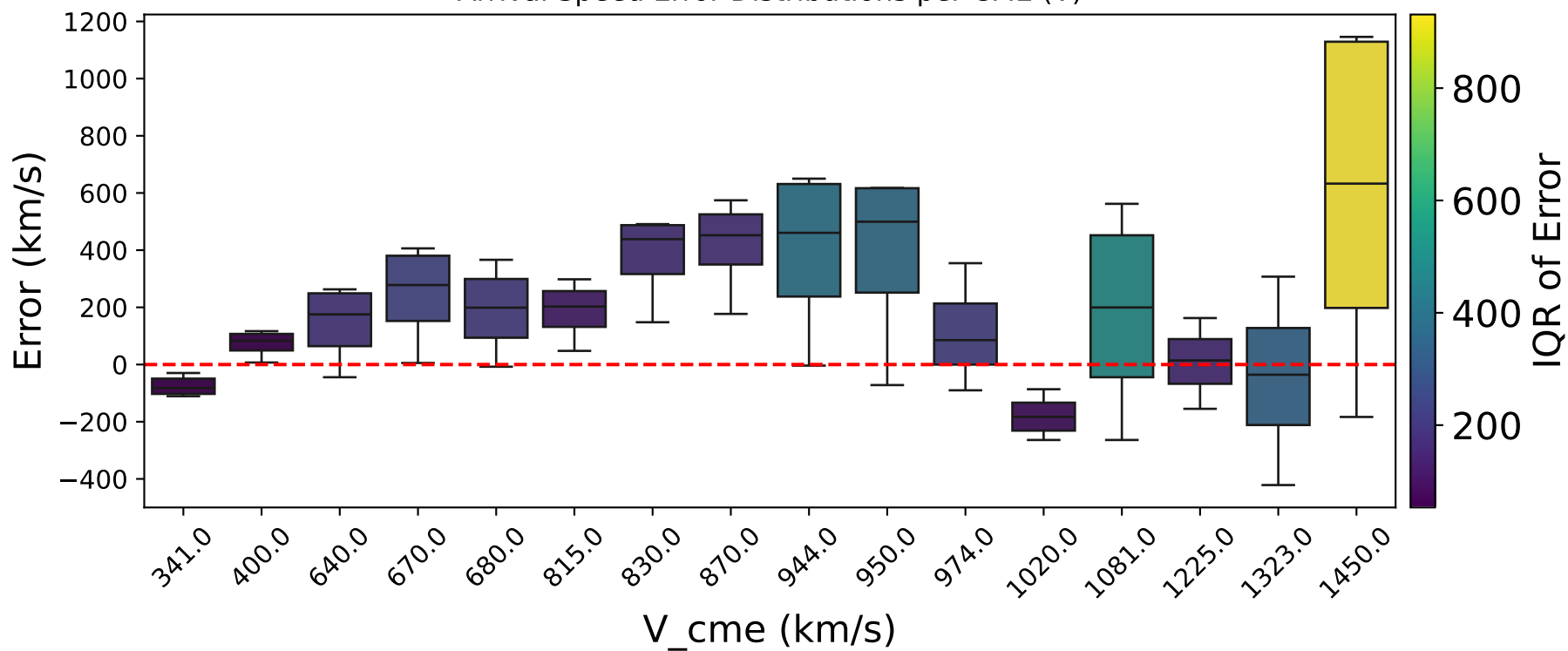
Arrival Speed Error Distributions per CME (V)
