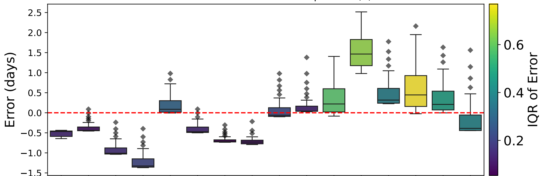
Transit Time Error Distributions per CME (V)
