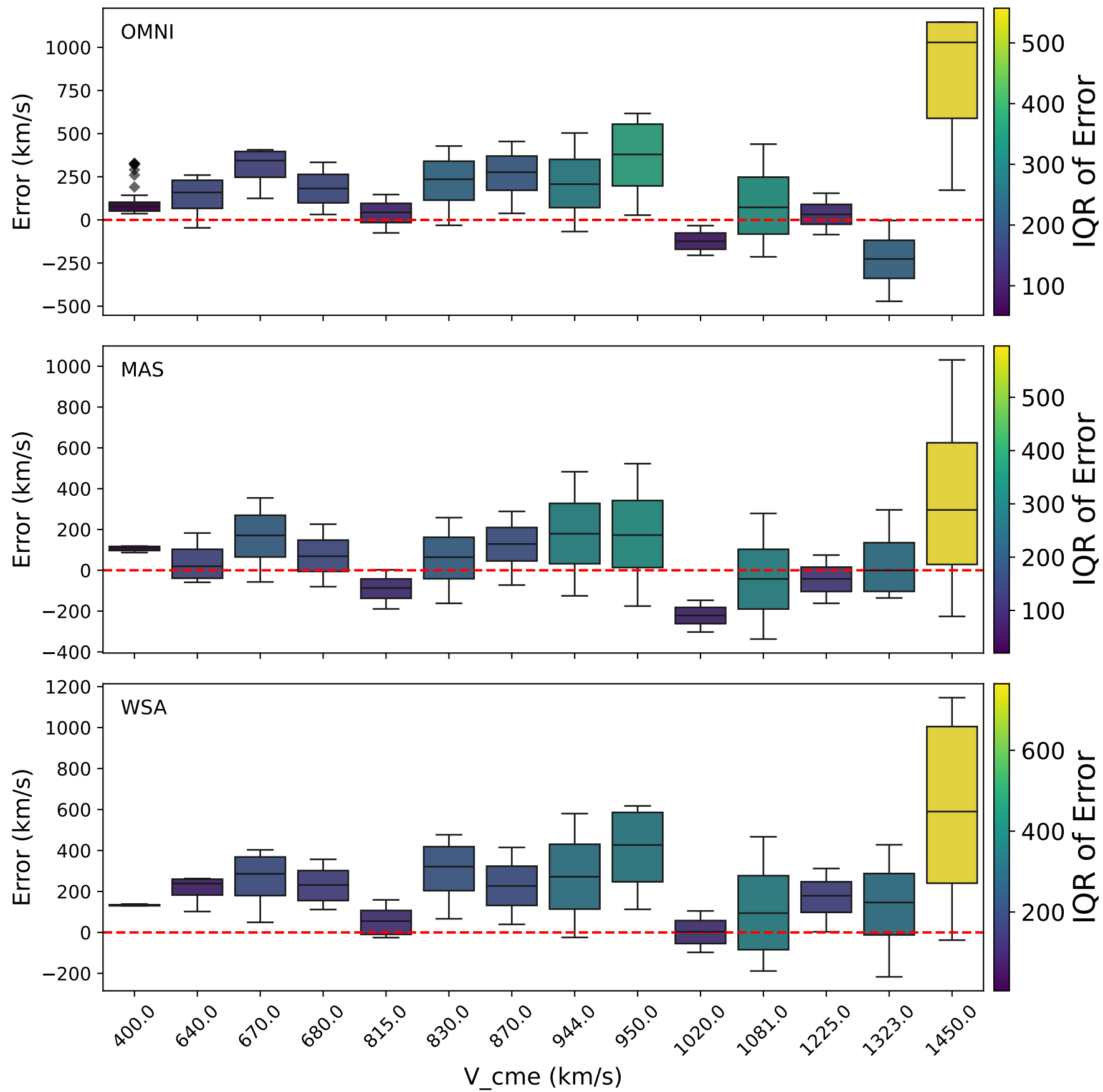
Arrival Speed Error Distributions vs CME Speed
