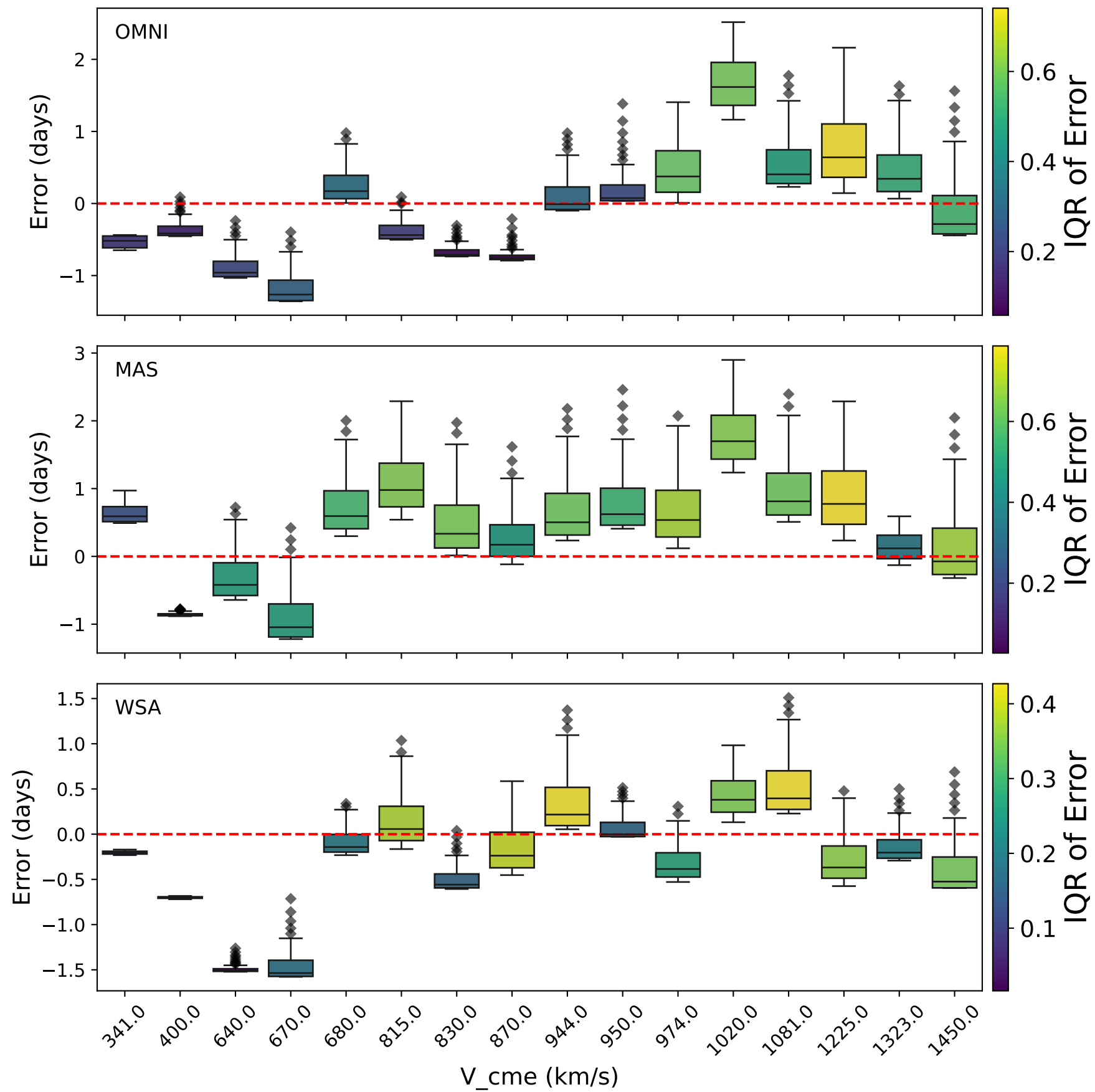
Transit Time Error Distributions vs CME Speed
