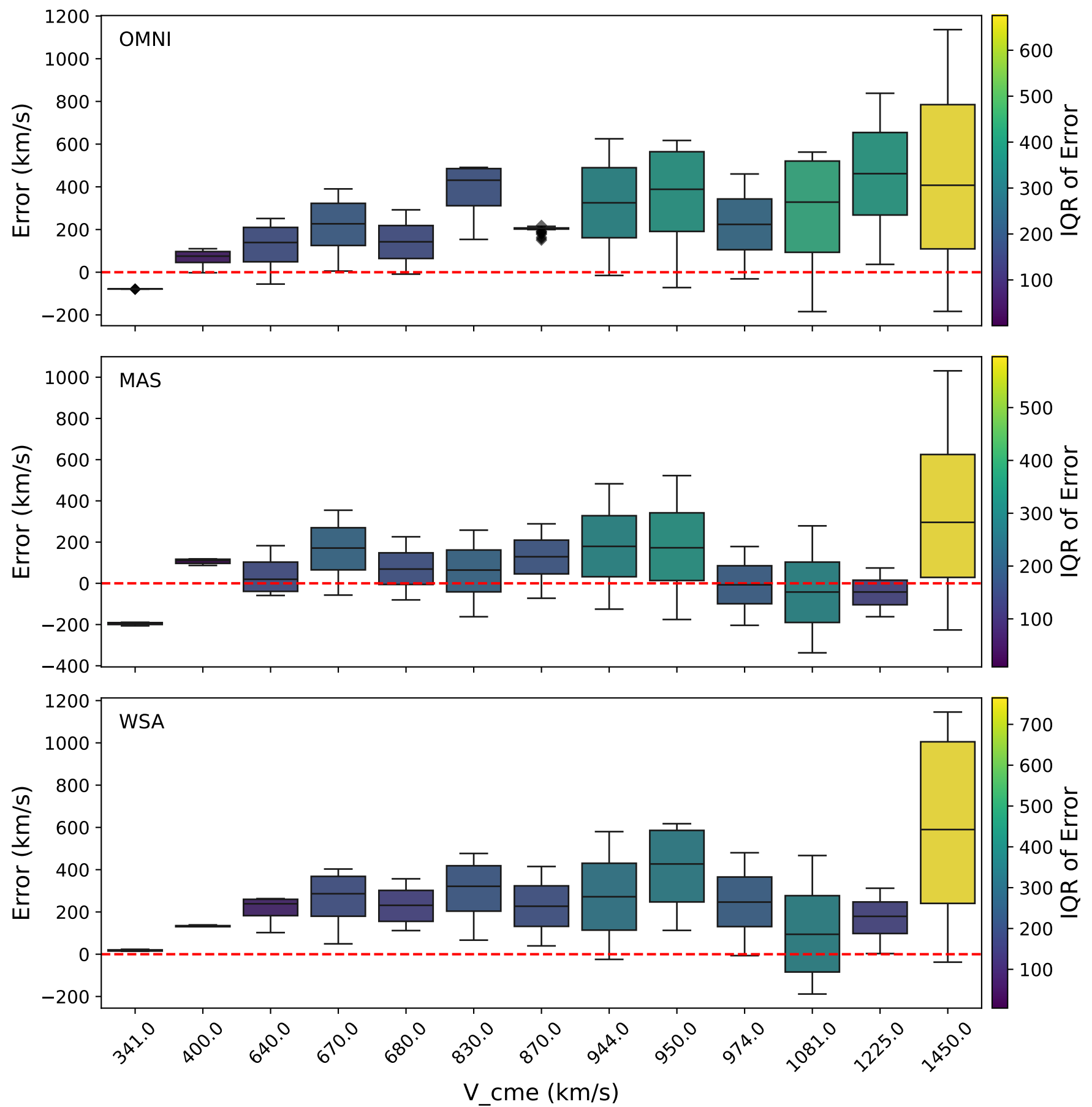
Arrival Speed Error Distributions vs CME Speed
