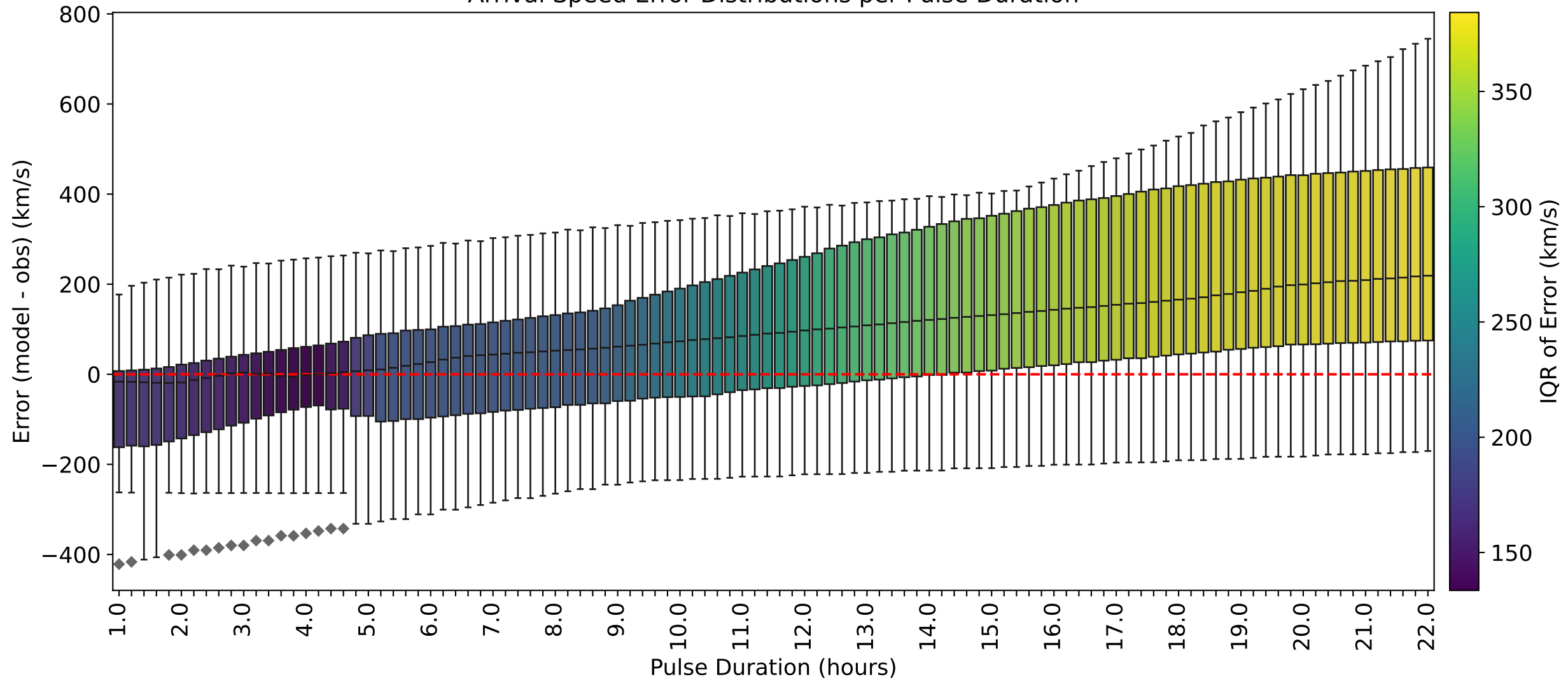
Arrival Speed Error Distributions per Pulse Duration
