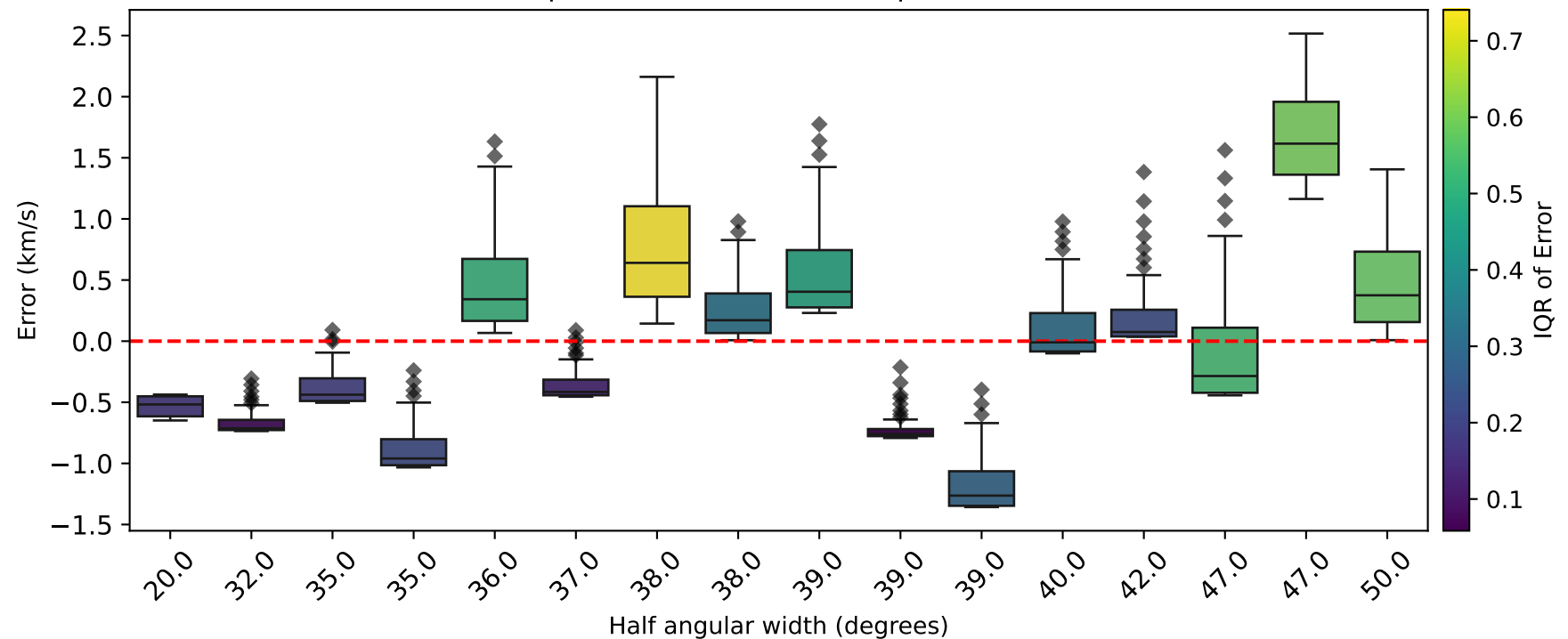
Arrival Speed Error Distributions per CME (Width)
