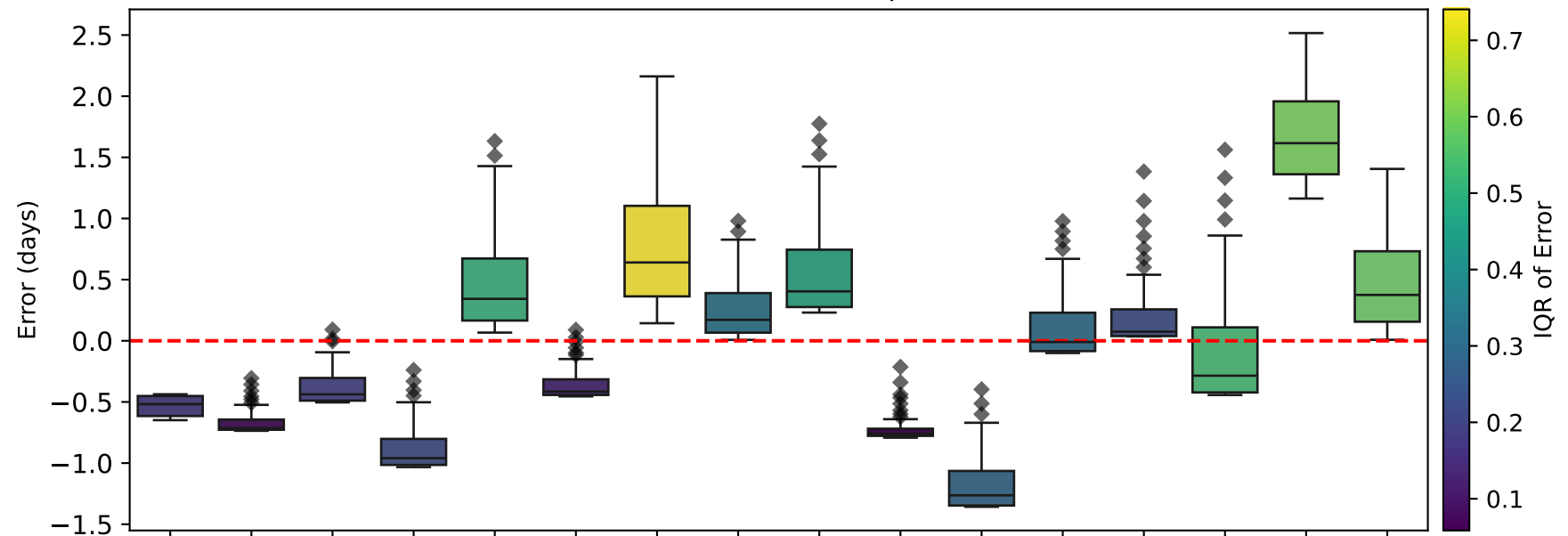
Transit Time Error Distributions per CME (Width)
