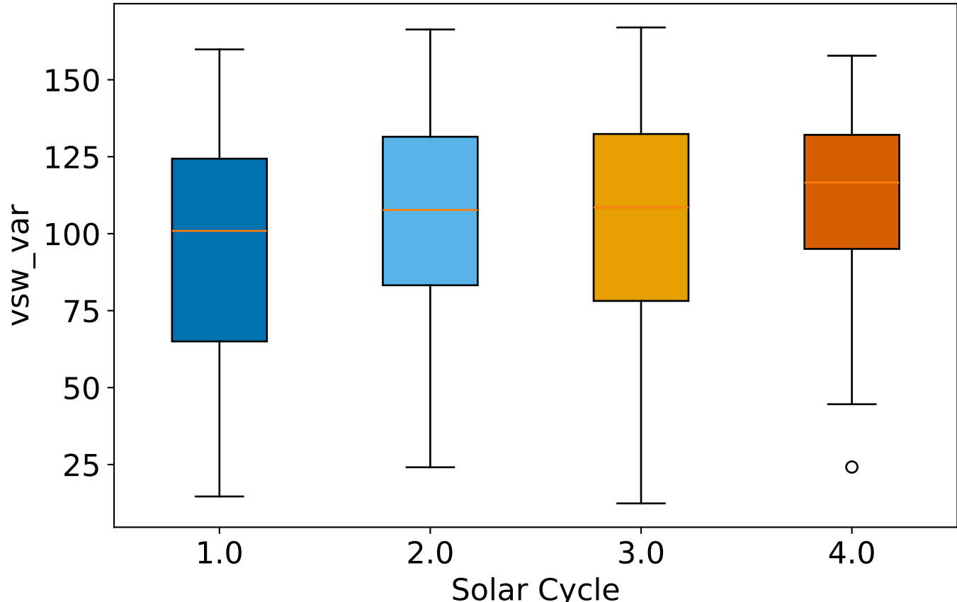
Solar wind variability per solar cycle
