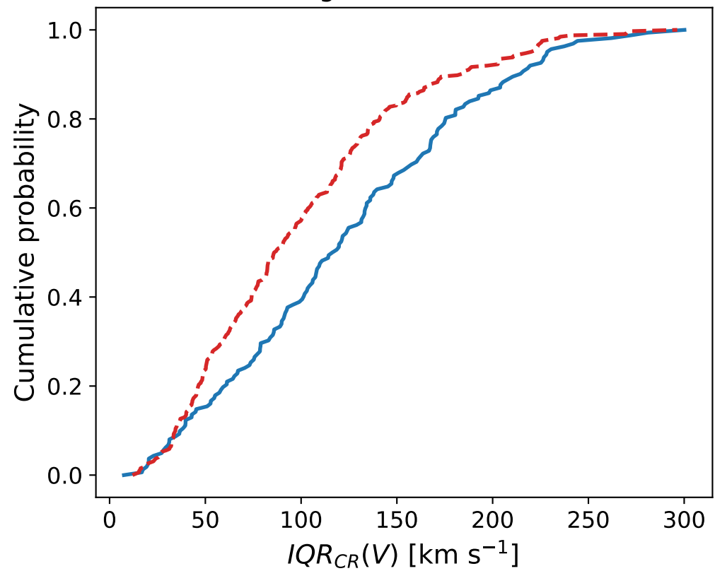
Average CME ( D=0.196 )
