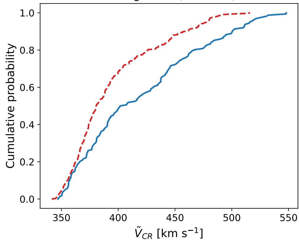
Average CME ( D=0.239 )
