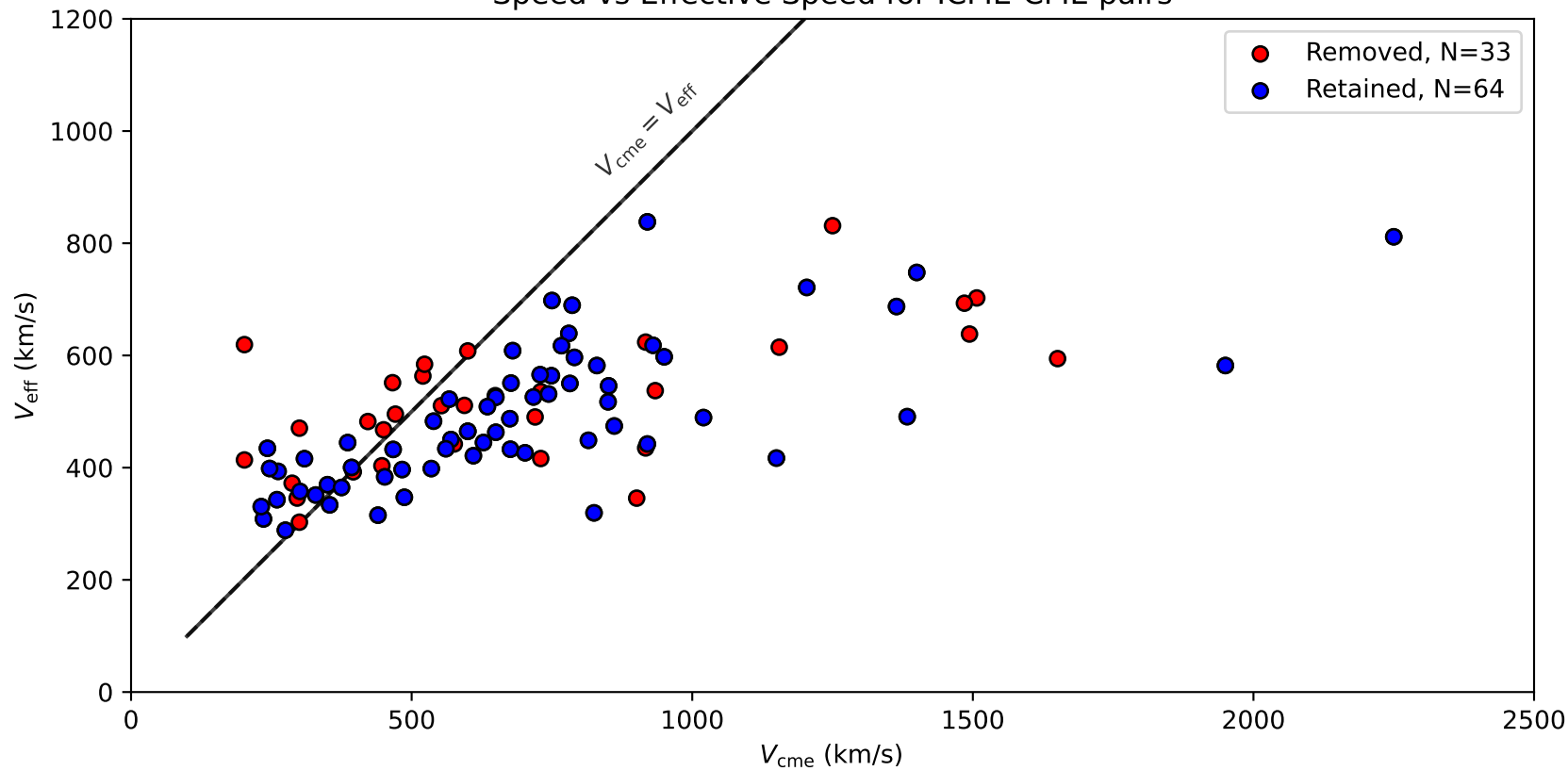
Speed vs Effective Speed for ICME-CME pairs
