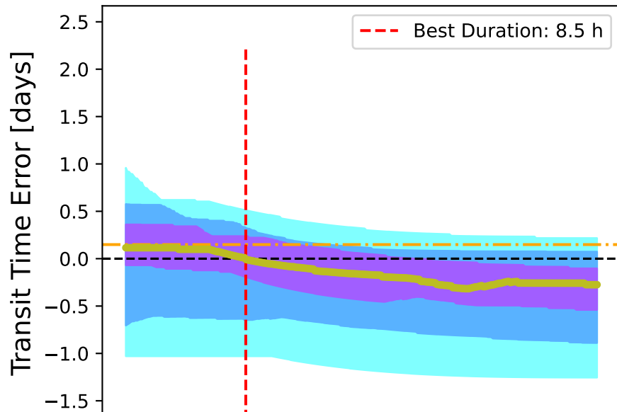
(c) MAS-recon
