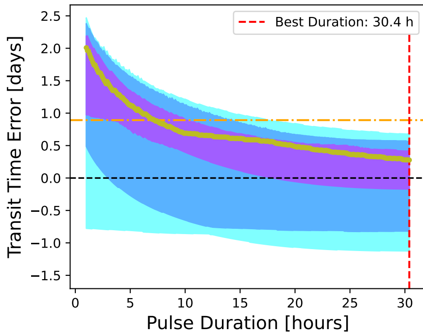
(c) MAS-recon
