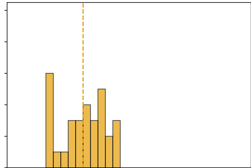
(b) OMNI-fcst
