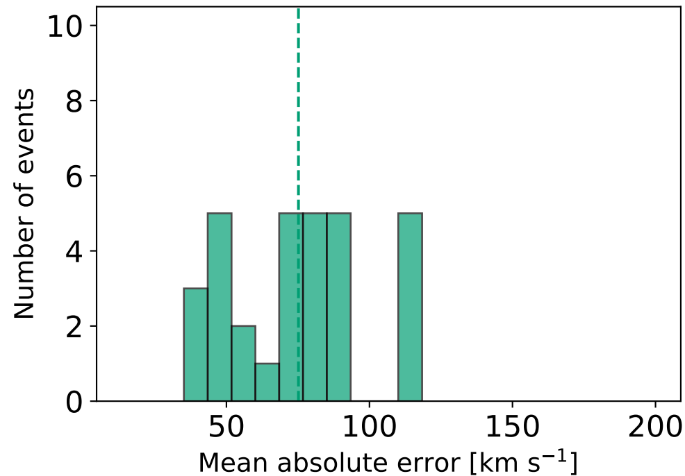
(c) MAS
