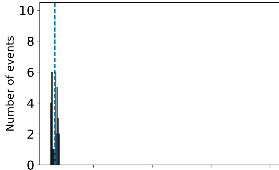
(a) OMNI-recon
