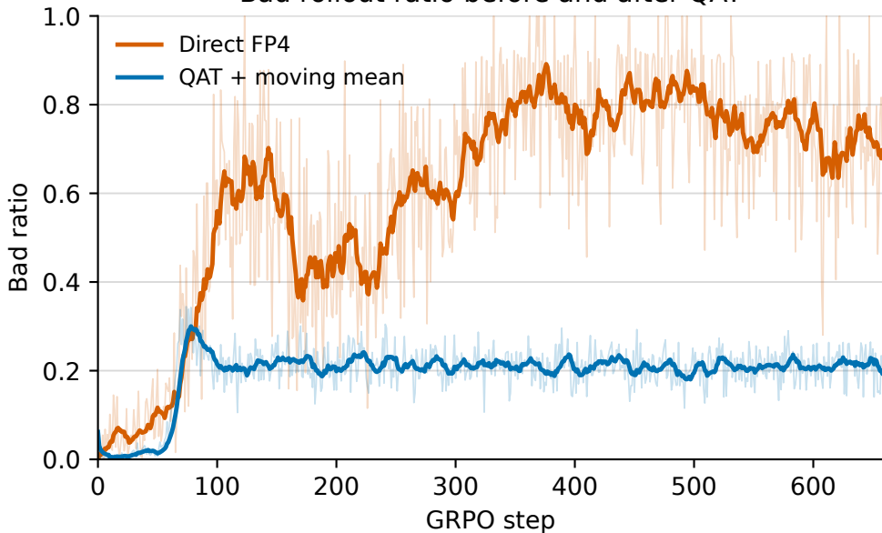
Bad rollout ratio before and after QAT
