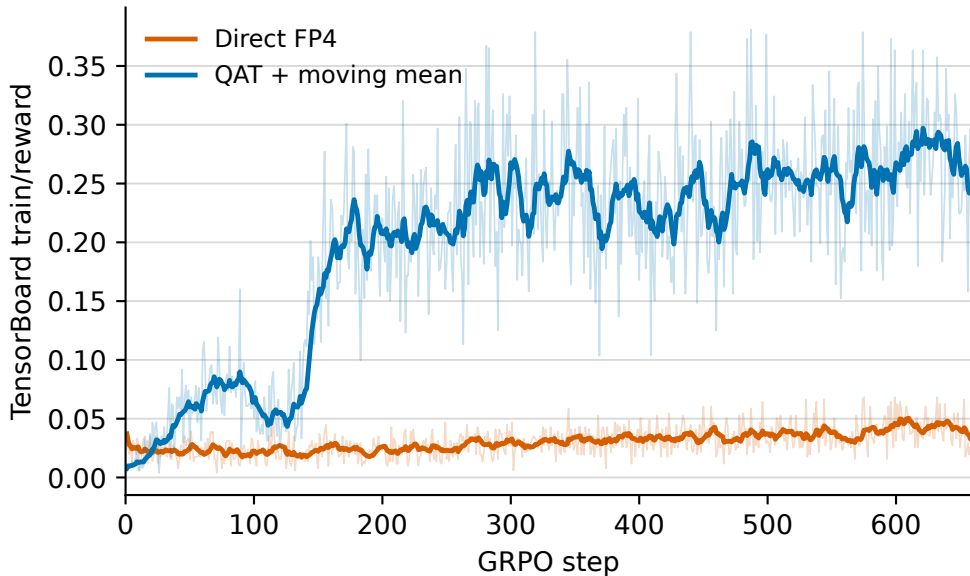
Training reward before and after QAT
