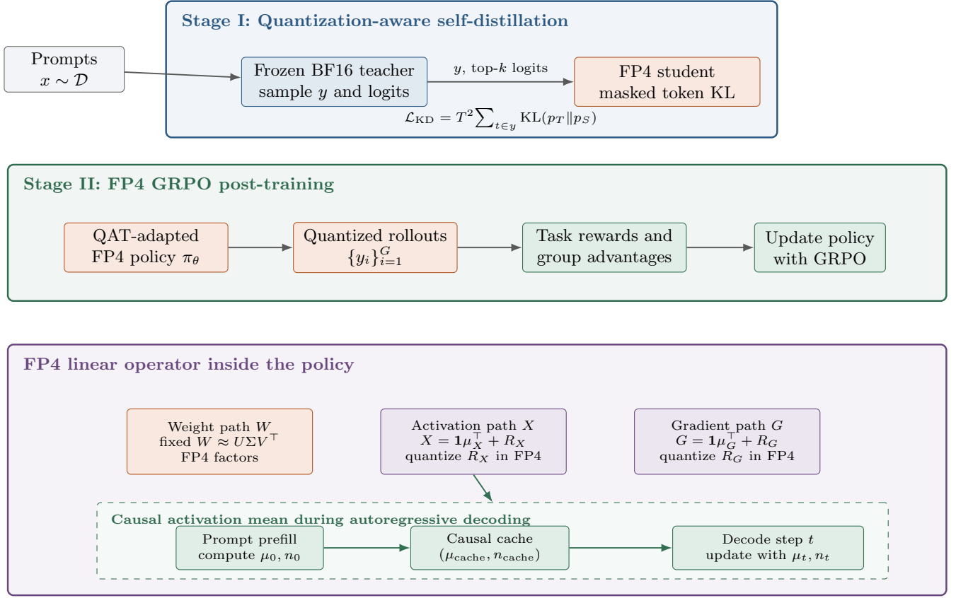
Figure 1: Overview of FP4 post-training. Stage I distills a BF16 teacher into an FP4 student on teacher-generated responses. Stage II uses the adapted FP4 policy to generate GRPO rollouts and updates it using group-relative rewards. Within the FP4 linear operator, weights follow the fixed SVD decomposition path, whereas activations and gradients are quantized after mean-residual decomposition; a causal moving-mean cache supplies the activation mean during autoregressive decoding.
