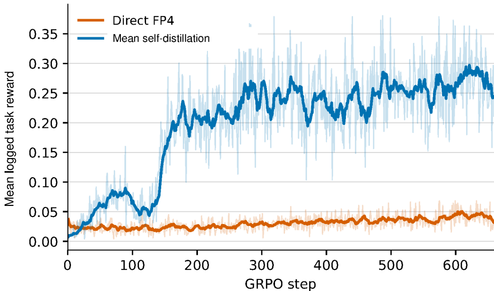
Mean logged task reward
