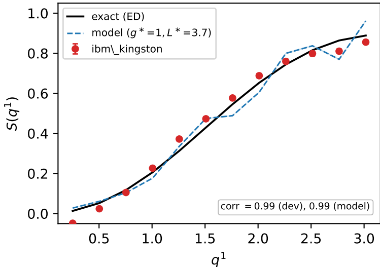
(a) structure factor, 101 qubits
