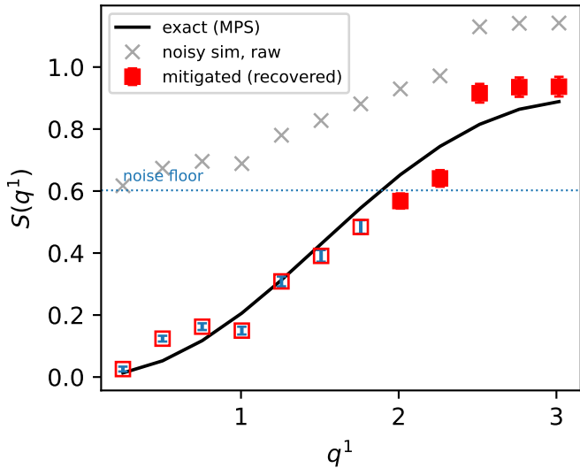
(a) structure factor, 101 qubits
