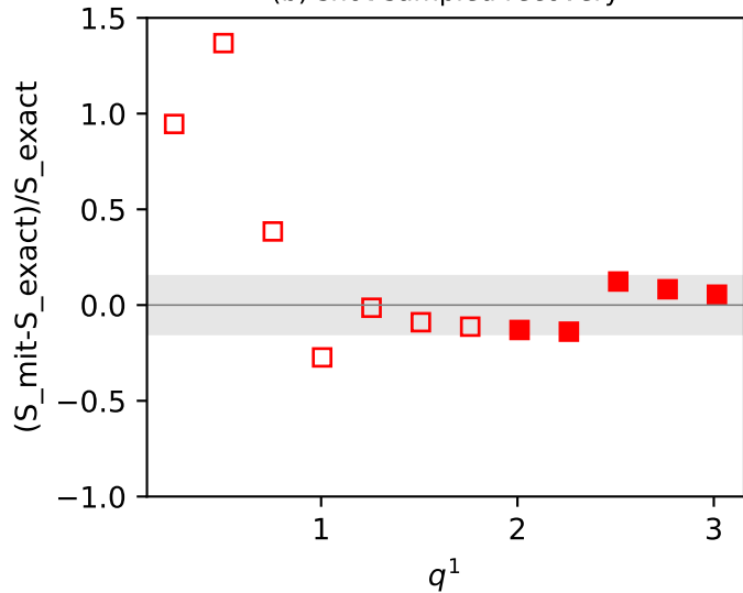
(b) shot-sampled recovery
