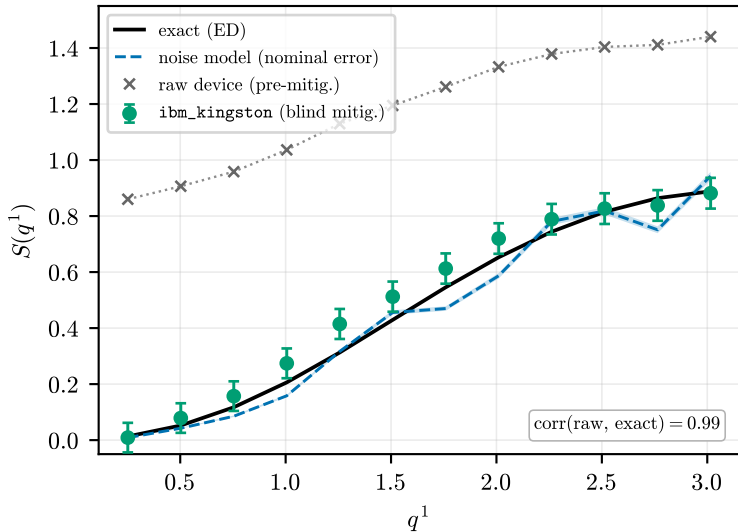
(a) structure factor, 101 qubits
