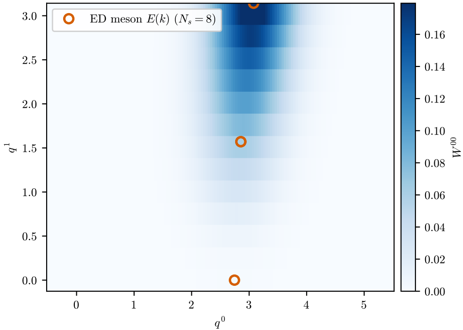
W_{\text{vac}}^{00}(q^0, q^1) (MPS, 101 qubits)
