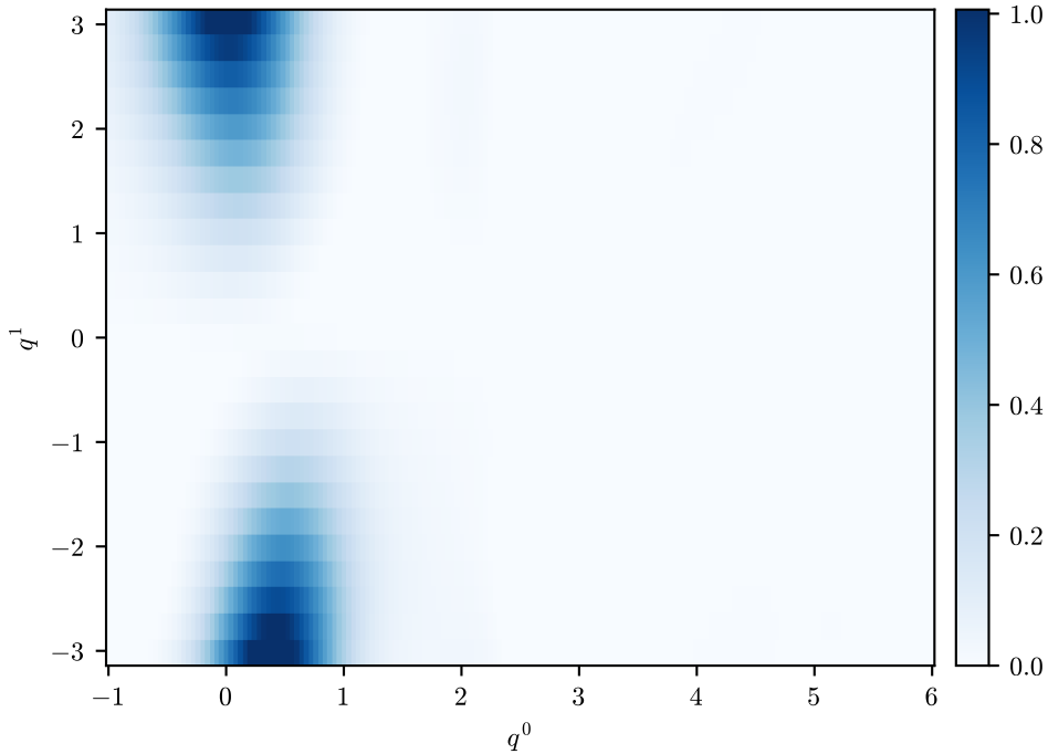
W^{00}(q^0, q^1) meson packet, k_0 = 1.26
