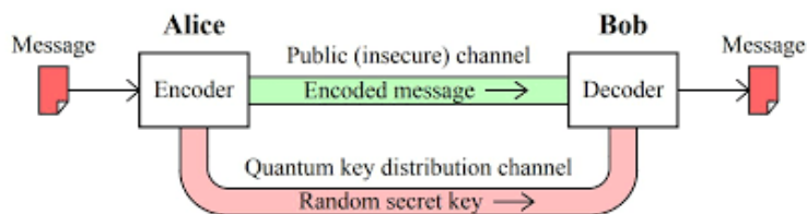
Figure 10: Quantum Key Distribution (QKD) Protocol. Alice sends a sequence of qubits to Bob, who measures them. They then compare their measurement bases over a classical channel to generate a secure, shared encryption key.
