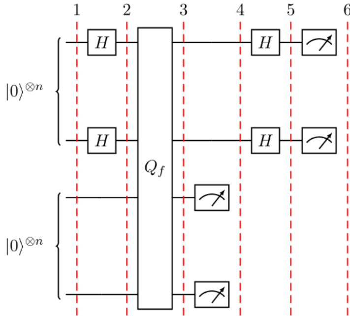
Figure 4: https://medium.com/@monitsharma/learn-quantum-computing-with-qiskit-simons-algorithm-8525adecd091
