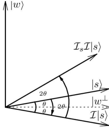
Figure 6: https://www.researchgate.net/figure/Geometric-visualization-of-Grovers-algorithm_fig147438604
