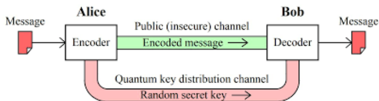
Figure 10: Illustration of Quantum Key Distribution (QKD) Protocol. Alice sends a sequence of qubits to Bob, who measures them. They then compare their measurement bases over a classical channel to generate a secure, shared encryption key.
