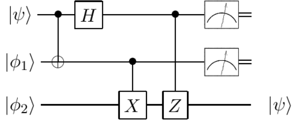
Figure 8: https://www.researchgate.net/figure/modified-quantum-teleportation-circuit_fig12_28663990
