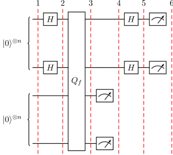
Figure 4: https://medium.com/@monitsharma/learn-quantum-computing-with-qiskit-simons-algorithm-8525adecd091
