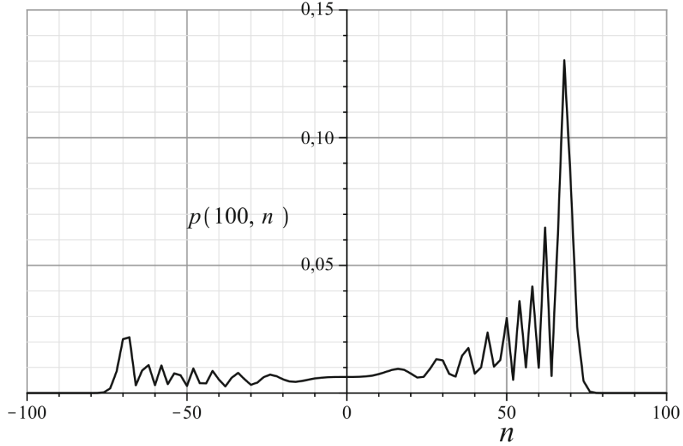
Figure 16: Probability distribution of a one-dimensional quantum walk using hadamard coin and initial position |0\rangle \otimes |0\rangle . [2]
