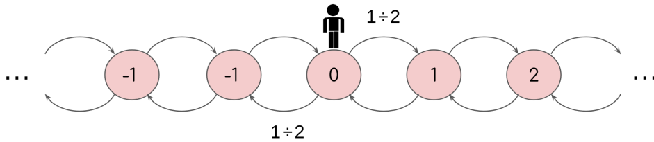
Figure 11: One Dimensional Discrete Time Random Walk with start position equal to zero.
