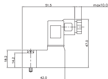
YSV20-DP-SC-CN1-*** Normally Closed
