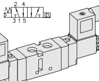
SF4200-IP-SC2-CN2-*** 2 4 3 1 5
